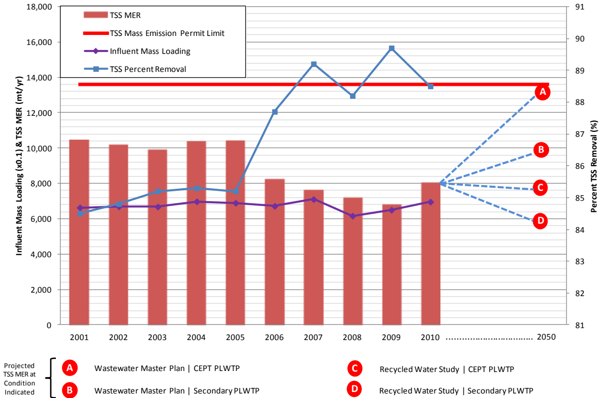
Figure B-4. Historical and Projected Point Loma Plant TSS MER (MER projections based on assumed effluent quality) PLWTP = Point Loma Wastewater Treatment Plant CEPT = Chemically-Enhanced Primary Treatment
