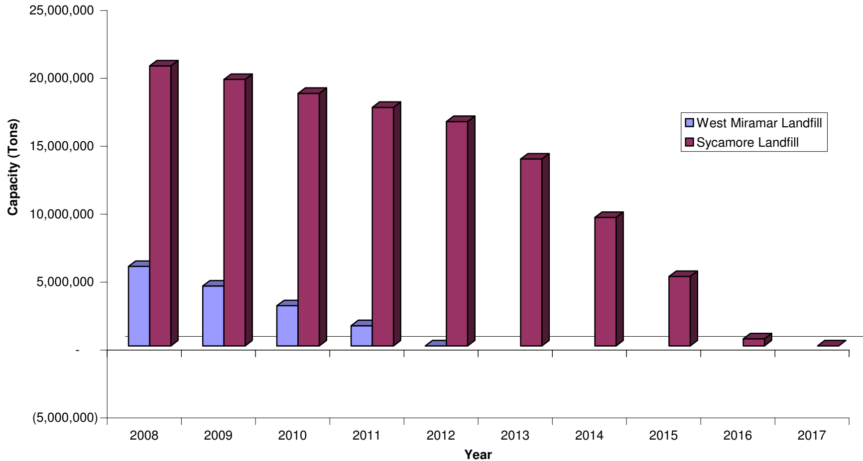
FIGURE 3-1 Projected Capacity Without West Miramar Landfill Height Increase & Without Sycamore Landfill Expansion (with Impact from City's Recycling & C&D Ordinances)
