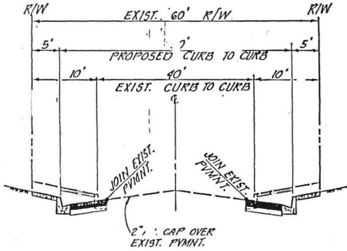
TYPICAL SECTION - SAN ANDRES DRIVE NO SCALE
