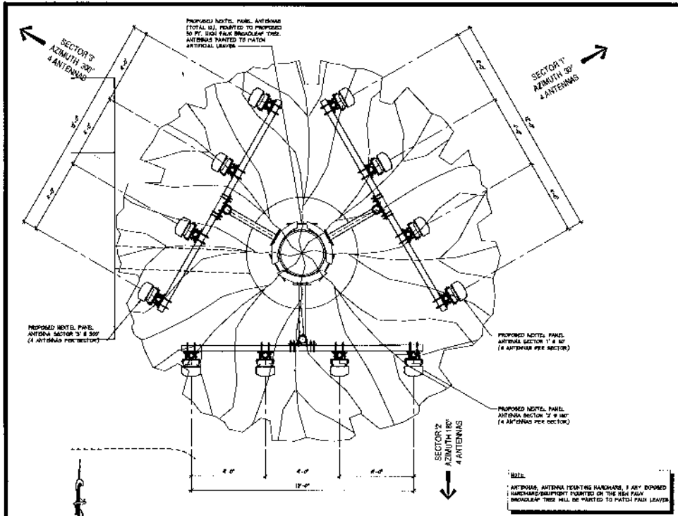
02 ANTENNA LAYOUT PLAN 1/4" = 1'-0"
