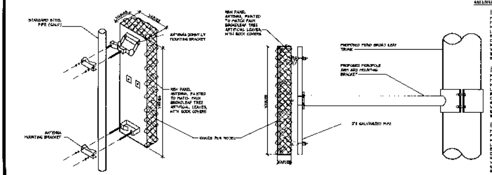
03 ANTENNA ATTACHMENT 1/4" = 1'-0"
