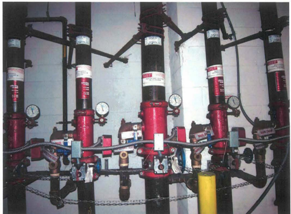
30) Typical of main fire risers in garage areas.
