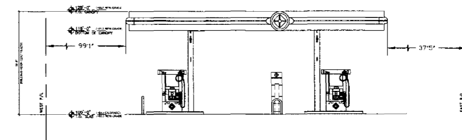
FUEL SYSTEM CANOPY SCALE: 1/8"=1'-0"
