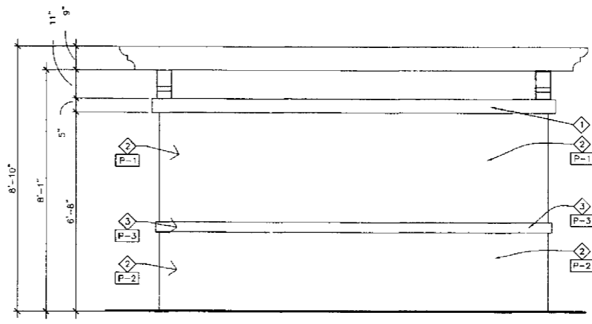
03 REAR ELEVATION SCALE: 1/2"=1'-0"
