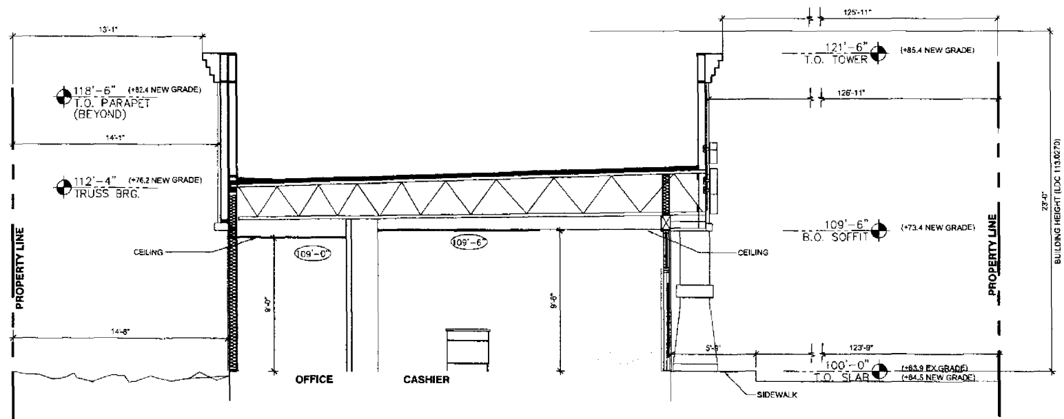
01 FRONT TO REAR BUILDING SECTION SCALE: 1/4"=1'-0"
