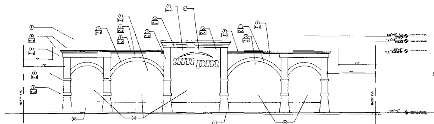
WEST ELEVATION "ARCO AM/PM" SCALE: 1/8"=1'-0"
