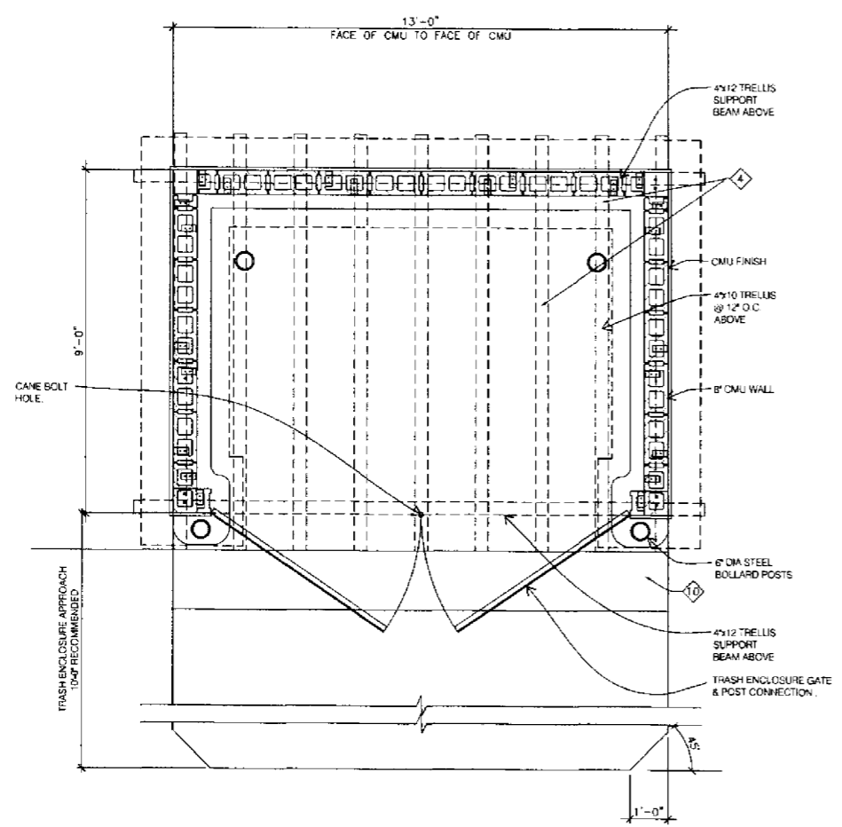
01 FOUNDATION & ROOF FRAMING PLAN SCALE: 1/2"=1'-0"
