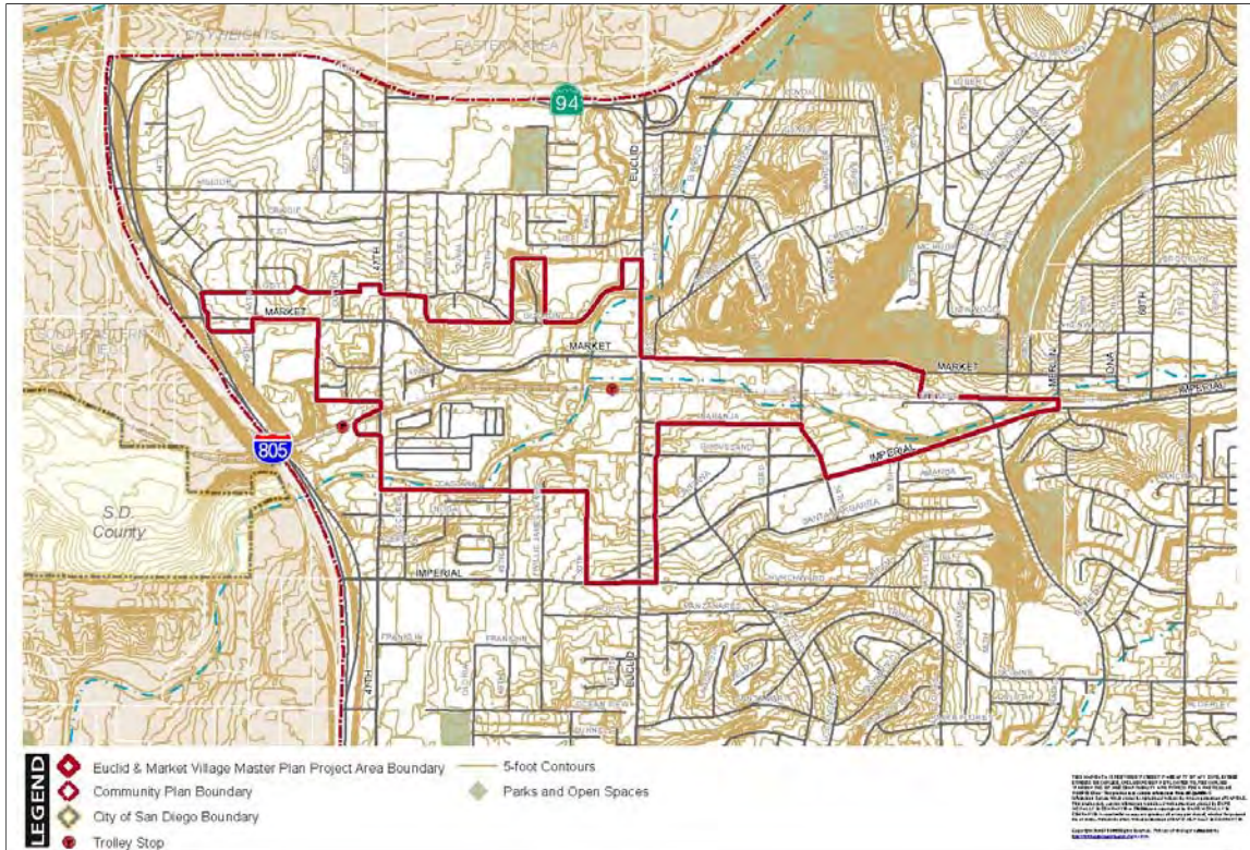
Figure 3-7 – Topography Map
