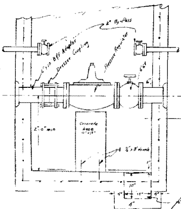
CROSS SECTION OF SIXTH AVE. AT THORN ST.
