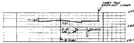
CROSS SECTION OF SIXTH AVE. AT THORN ST.
