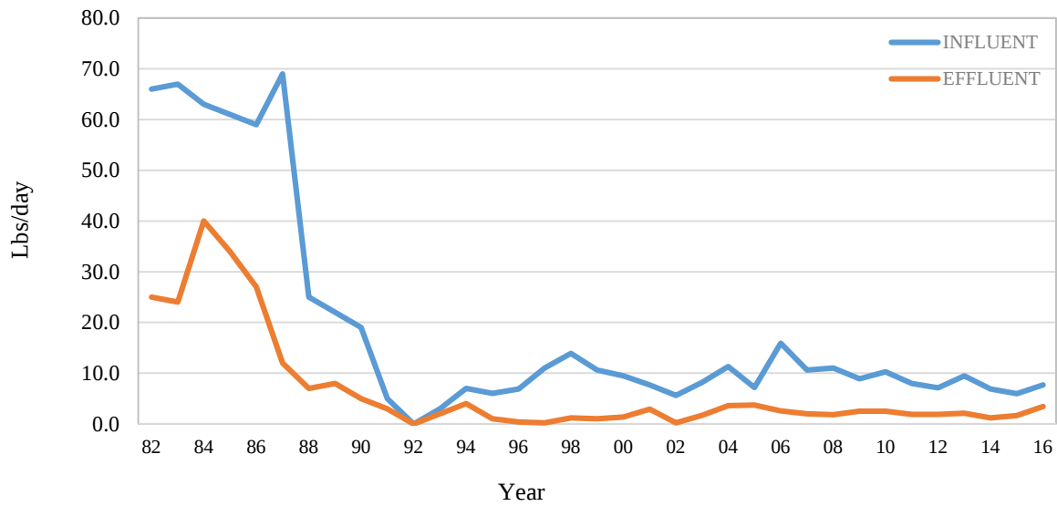
Figure 5.2-3 Chromium Point Loma Influent / Effluent History
