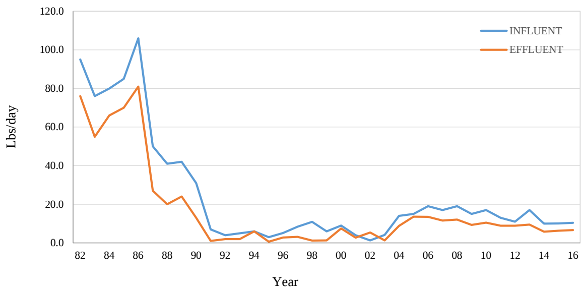
Figure 5.2-6 Nickel Point Loma Influent / Effluent History
