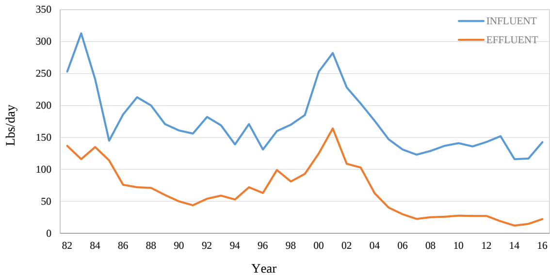
Figure 5.2-4 Copper Point Loma Influent / Effluent History
