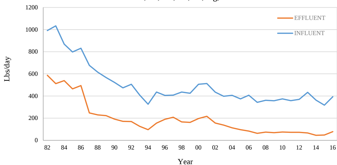
Figure 5.2-1 Point Loma Influent / Effluent Metals Total of Cd, Cr, Cu, Pb, Ni, Ag, Zn
