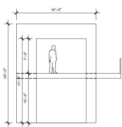
FRONT ELEVATION
