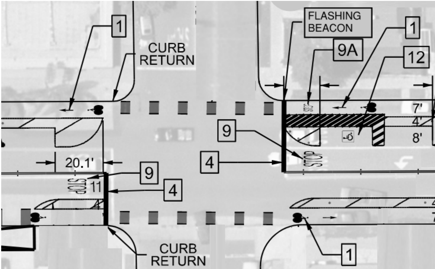
Flashing Beacon Intersection
