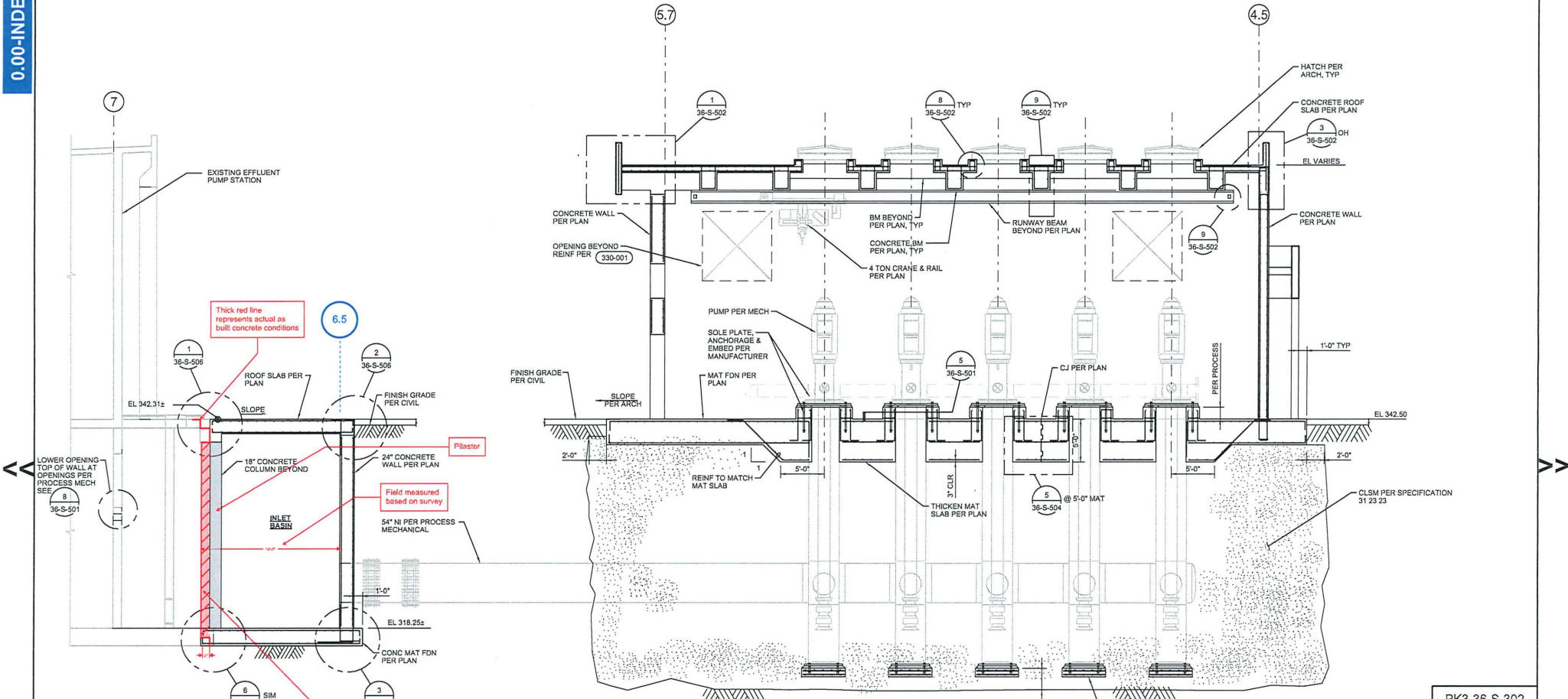
A SECTION 3/16"=1'-0" 36-S-130
