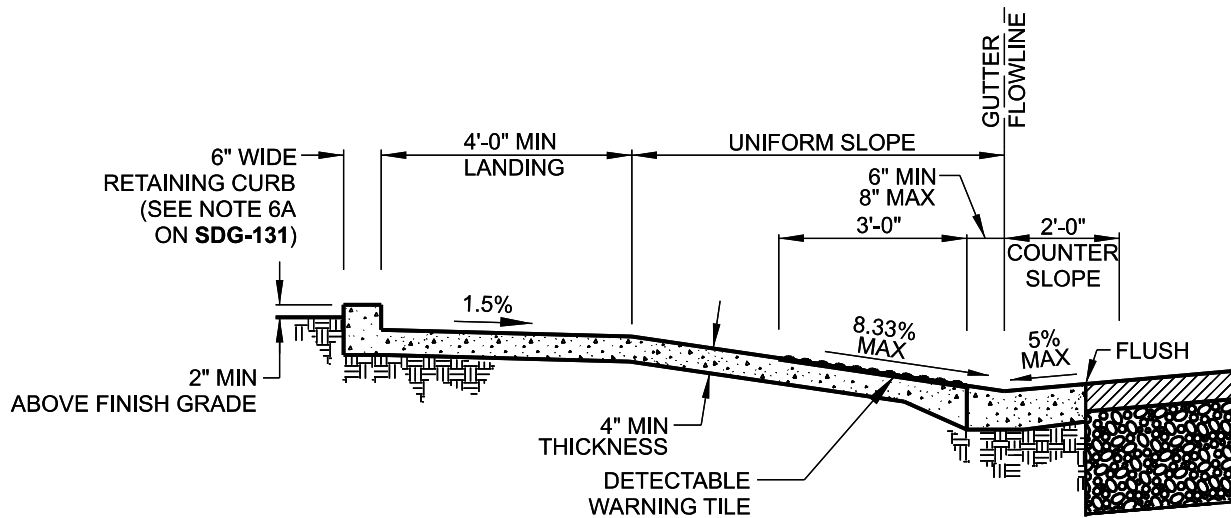
SECTIONS A & A1
