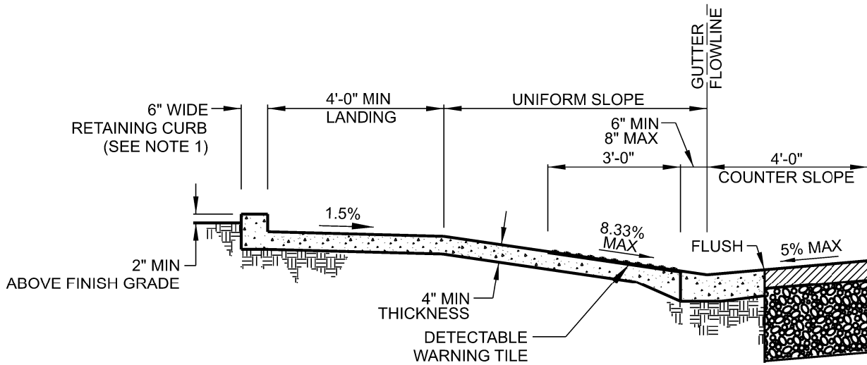
SECTION B-B
