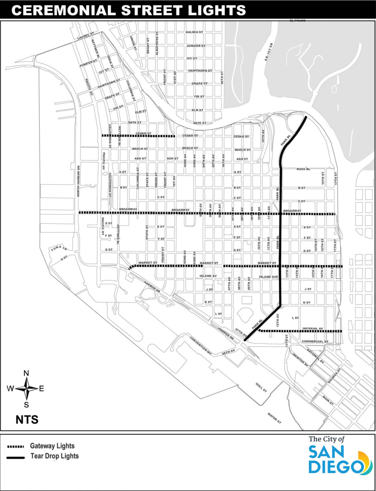
FIGURE 3-32 CEREMONIAL STREET LIGHTS
