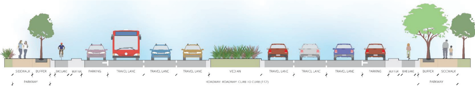
FIGURE 2-29 SIX-LANE URBAN MAJOR SECTION VIEW (OPTION C4)
