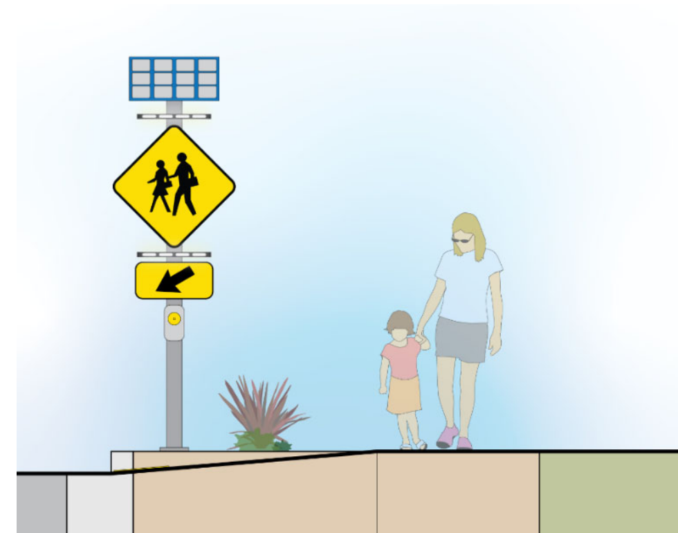
FIGURE 5-53 RECTANGULAR RAPID FLASHING BEACON SECTION VIEW
