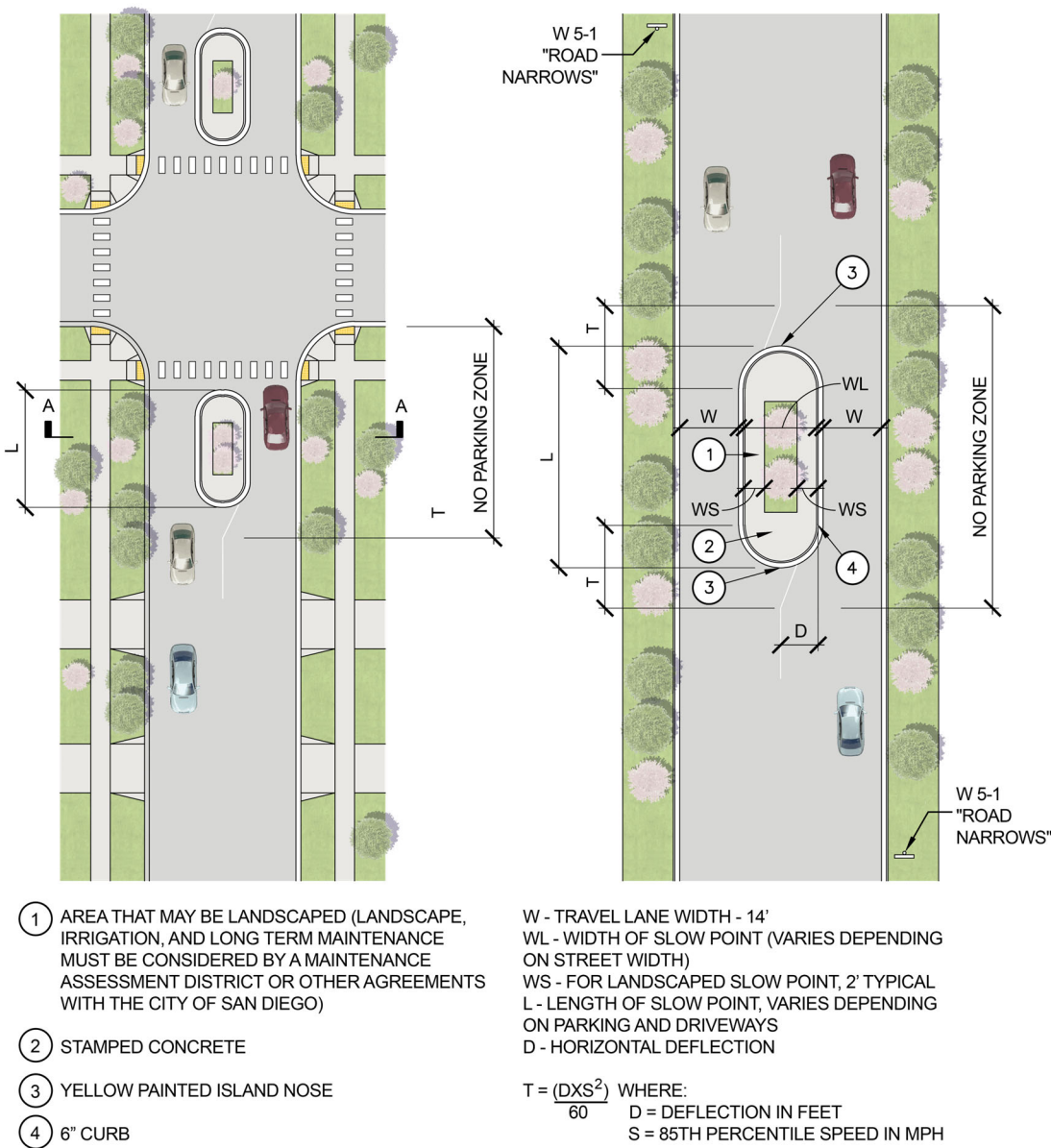
FIGURE 5-7 MEDIAN SLOW POINT PLAN VIEW
