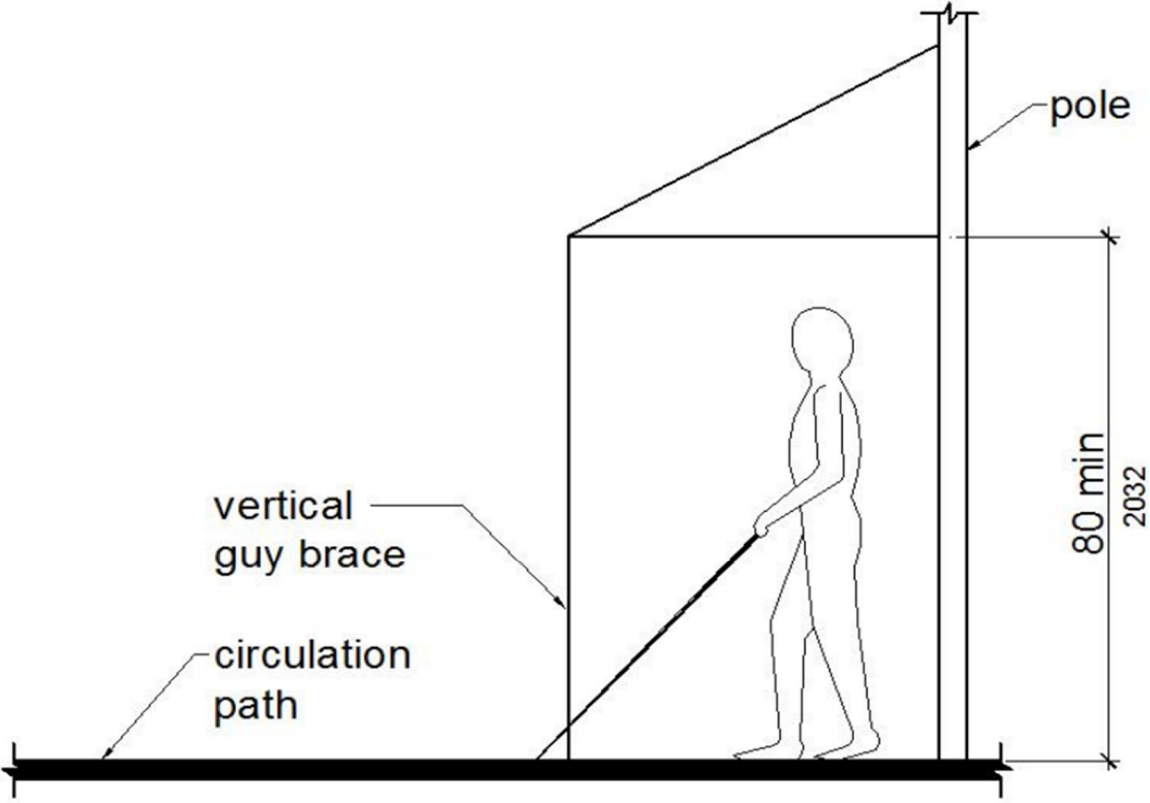
FIGURE 3-34 GUY BRACES
