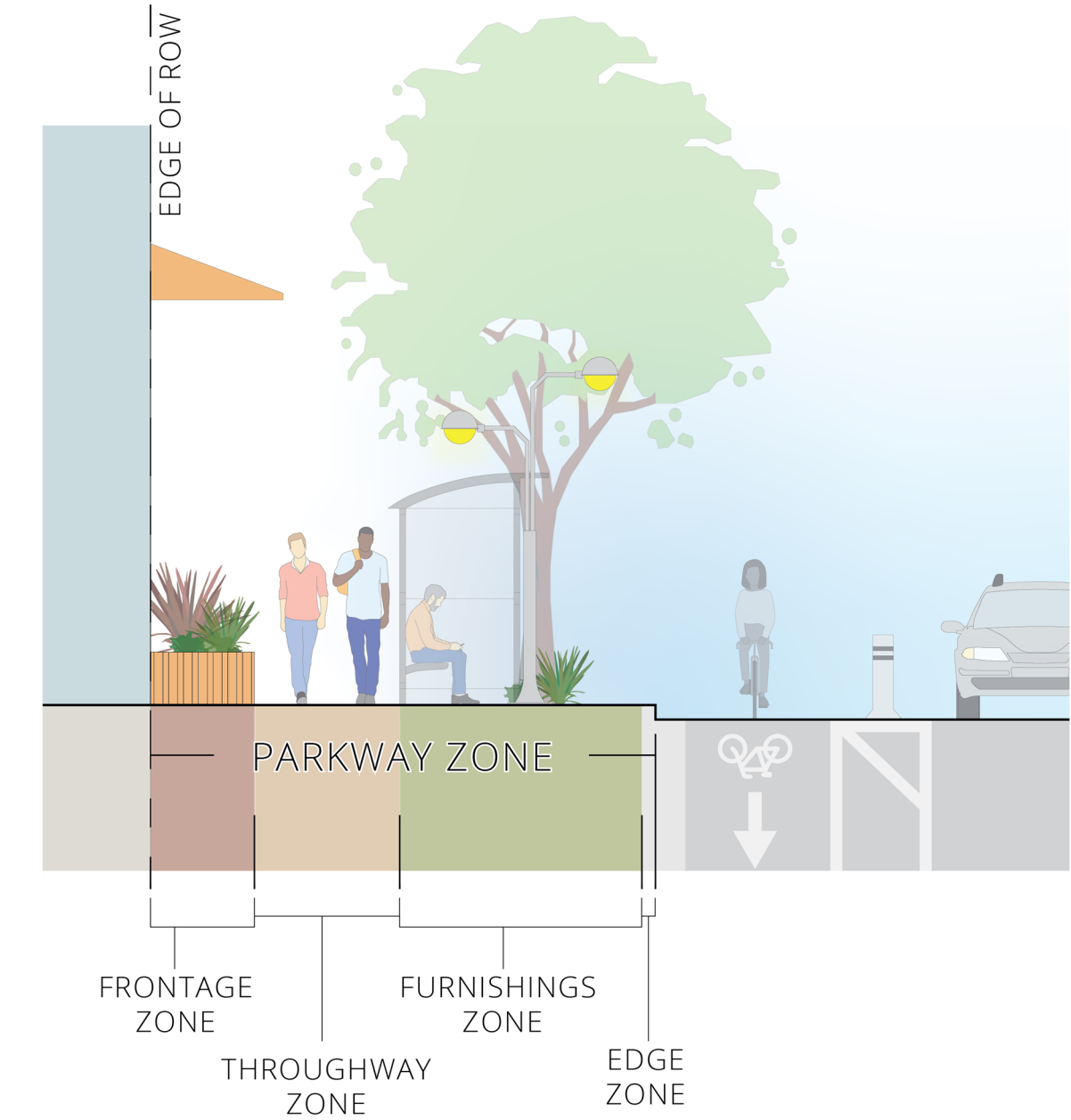
FIGURE 3-12 THE PARKWAY ZONES
