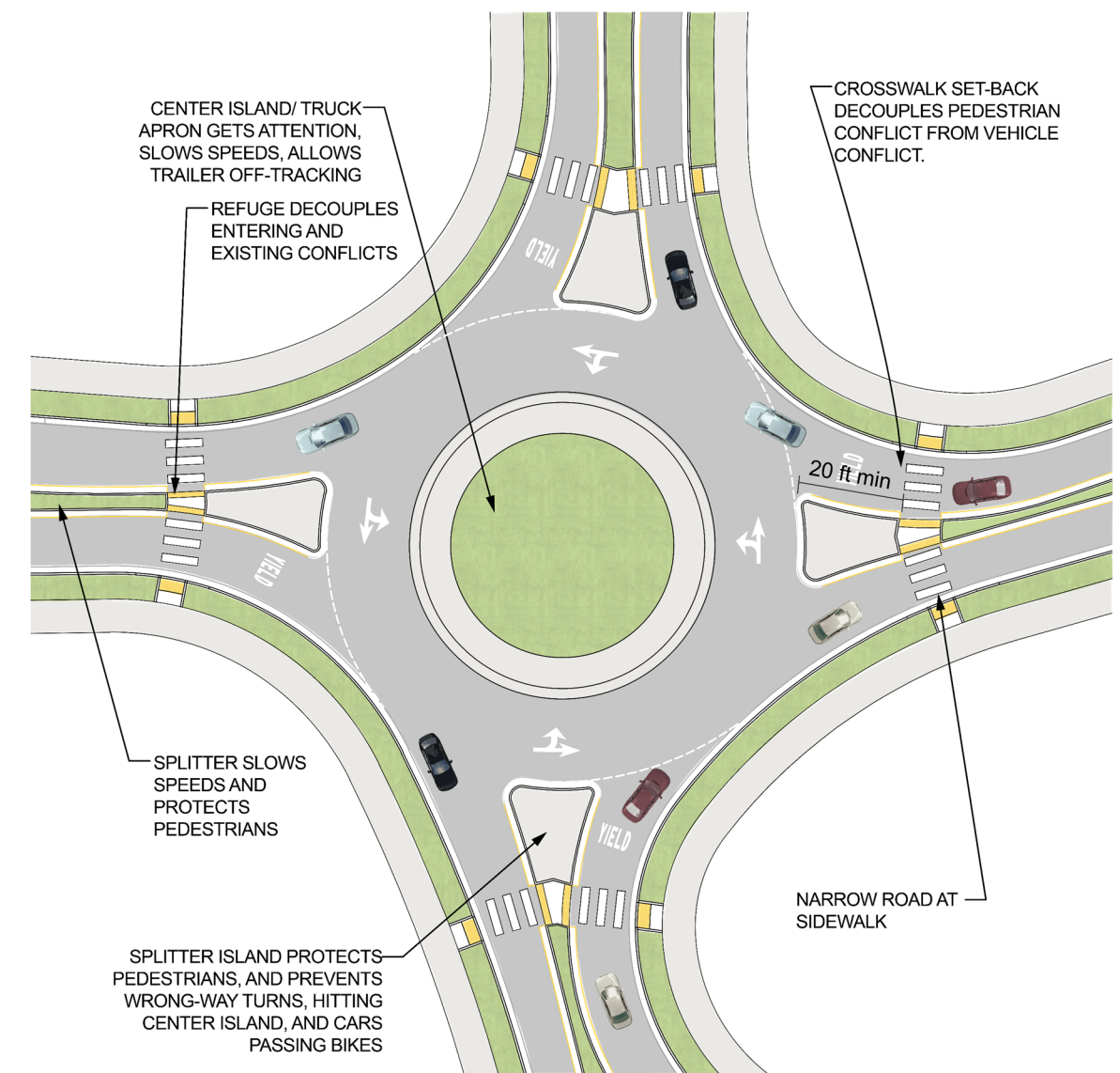
FIGURE 6-29 ROUNDABOUT
