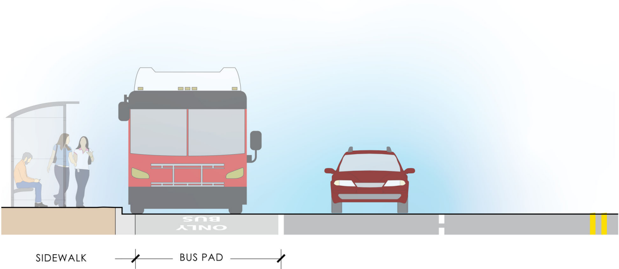
FIGURE 5-26 BUS PAD THROUGH THE LOCATION SECTION VIEW
