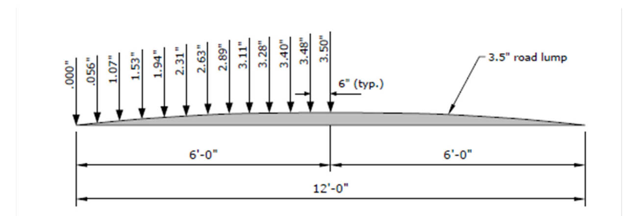
FIGURE 5-61 ROAD LUMP SECTION B-B
