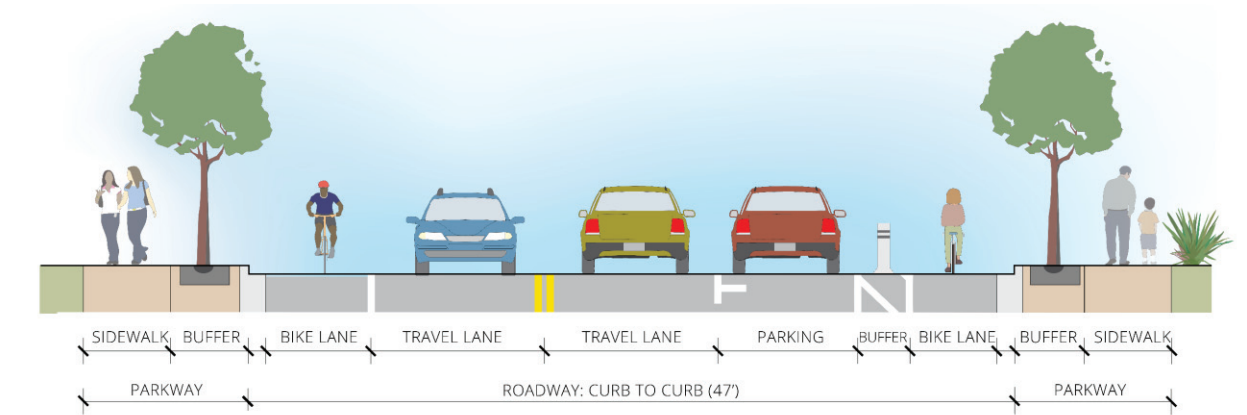
FIGURE 2-11 COMMERCIAL LOCAL STREET SECTION VIEW (OPTION C2)
