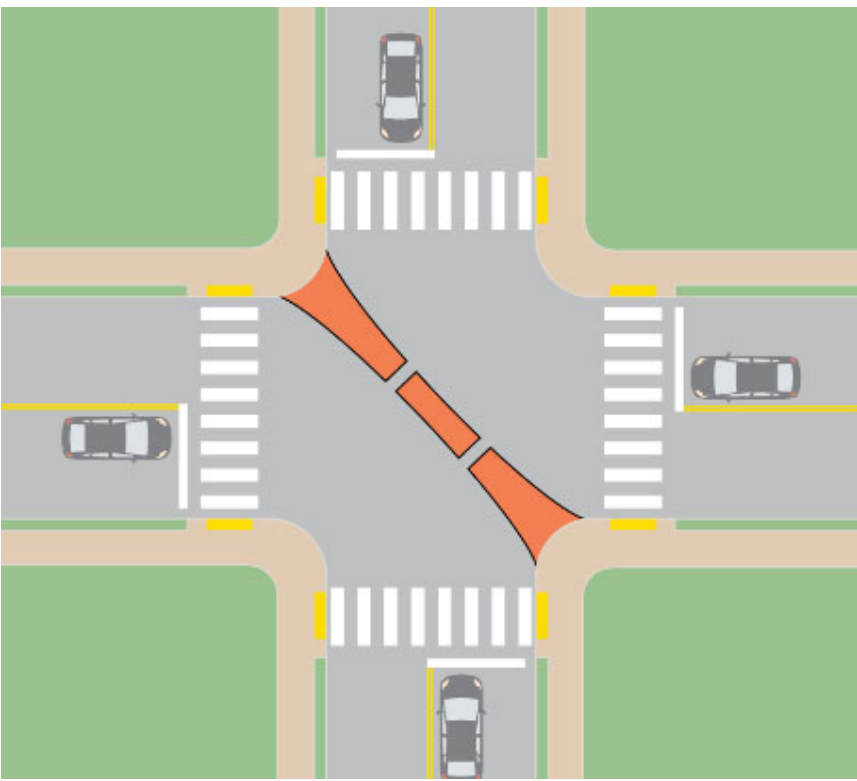
FIGURE 5-76 DIAGONAL DIVERTER
