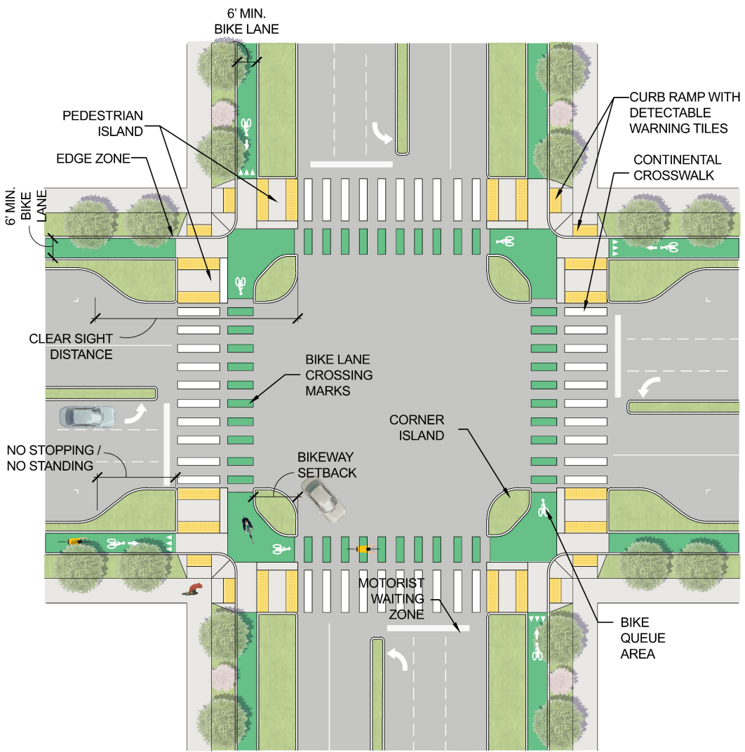
FIGURE 6-9 PROTECTED INTERSECTION
