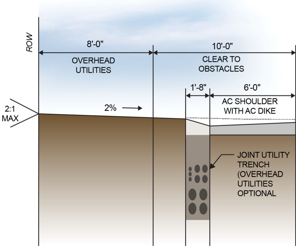
FIGURE 3-24 RP-1: 12' RURAL PARKWAY
