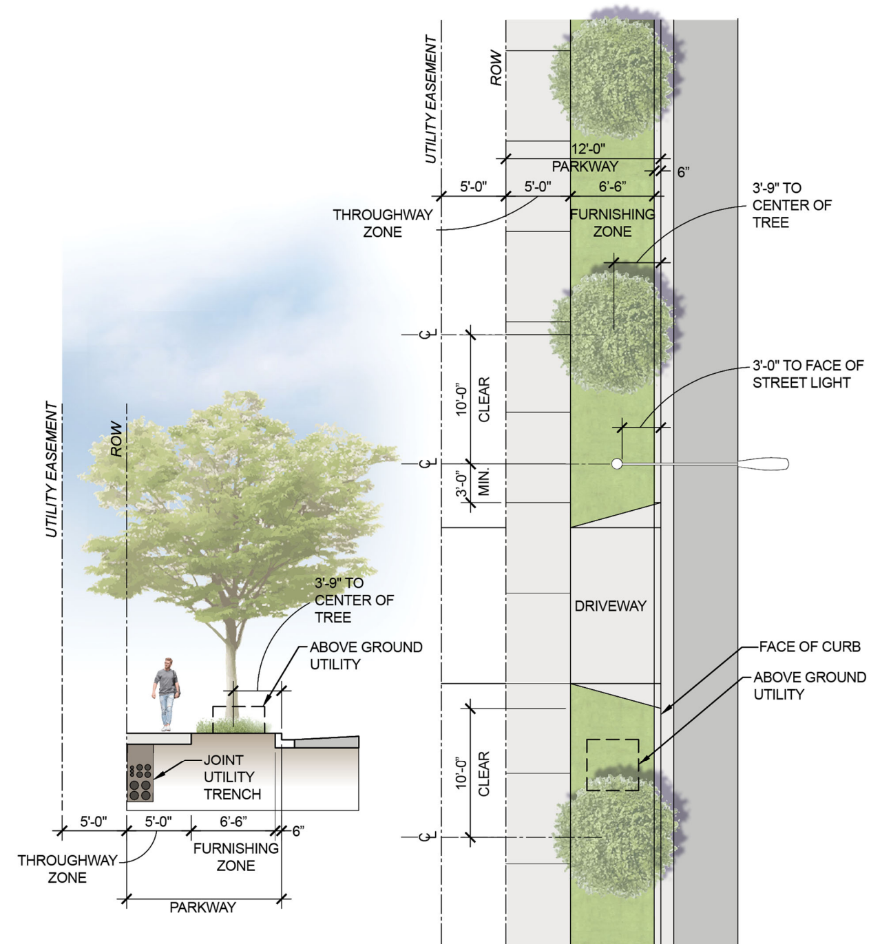
FIGURE 3-15 UP-3: 12' PARKWAY NON-CONTIGUOUS SIDEWALK
