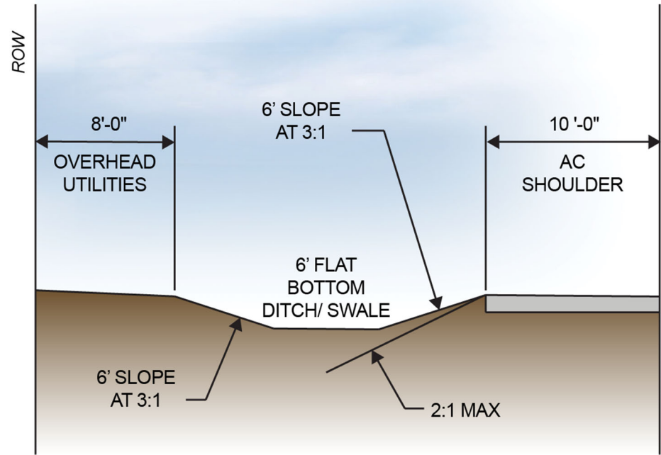
FIGURE 3-27 RP-4: 26' RURAL PARKWAY
