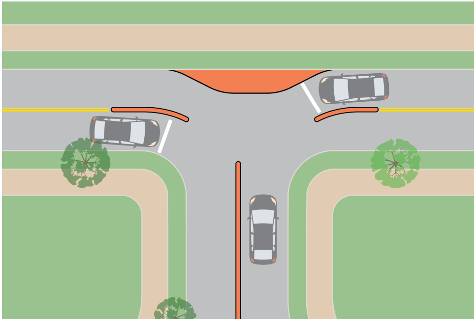
FIGURE 5-73 REALIGNED T-INTERSECTION
