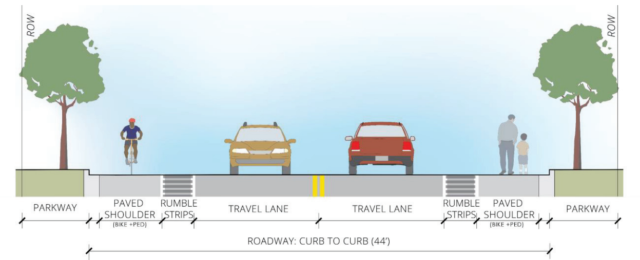
FIGURE 2-35 RURAL COLLECTOR ROAD SECTION VIEW (OPTION C2)
