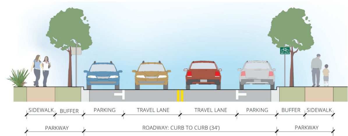
FIGURE 2-15 TWO-LANE SUB-COLLECTOR SECTION VIEW (OPTION C2)
