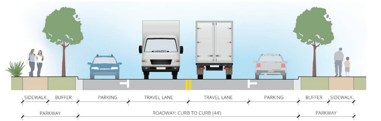
FIGURE 2-13 INDUSTRIAL LOCAL STREET SECTION VIEW (OPTION C1)
