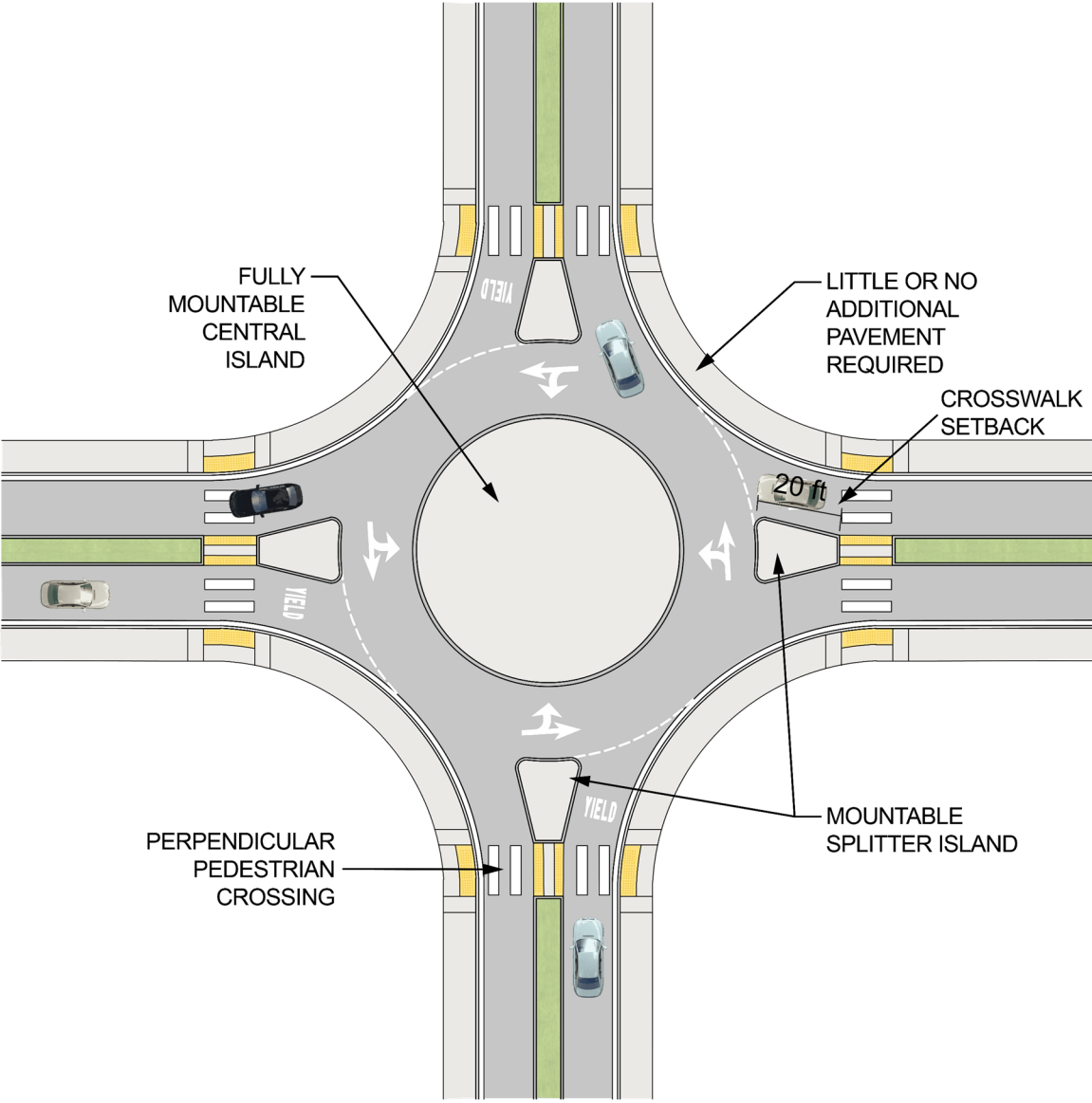
FIGURE 6-30 MINI-ROUNDAABOUT
