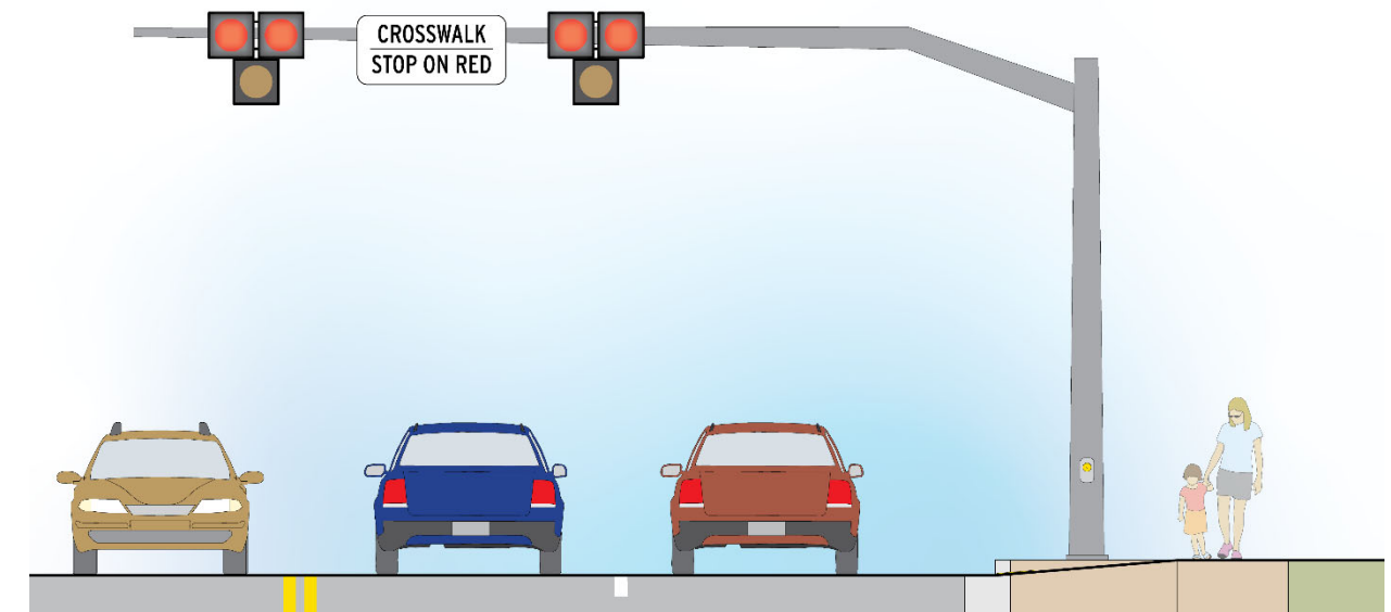
FIGURE 5-55 PEDESTRIAN HYBRID BEACON SECTION VIEW
