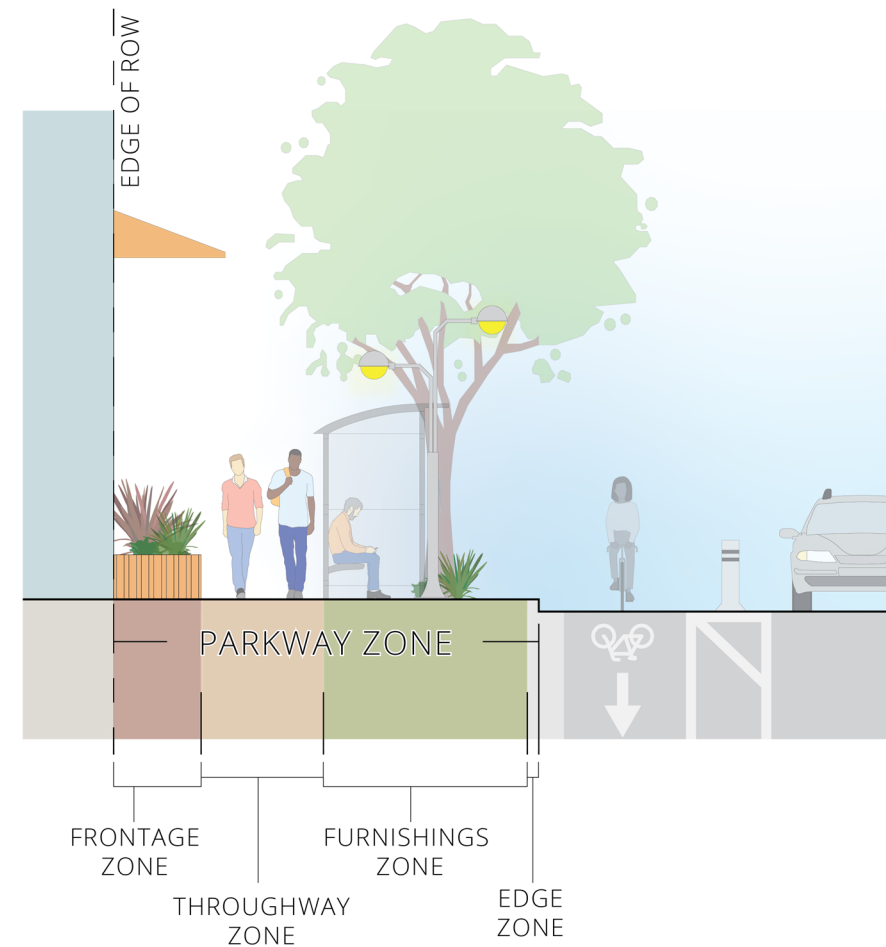
FIGURE 3-2 PARKWAY ZONES
