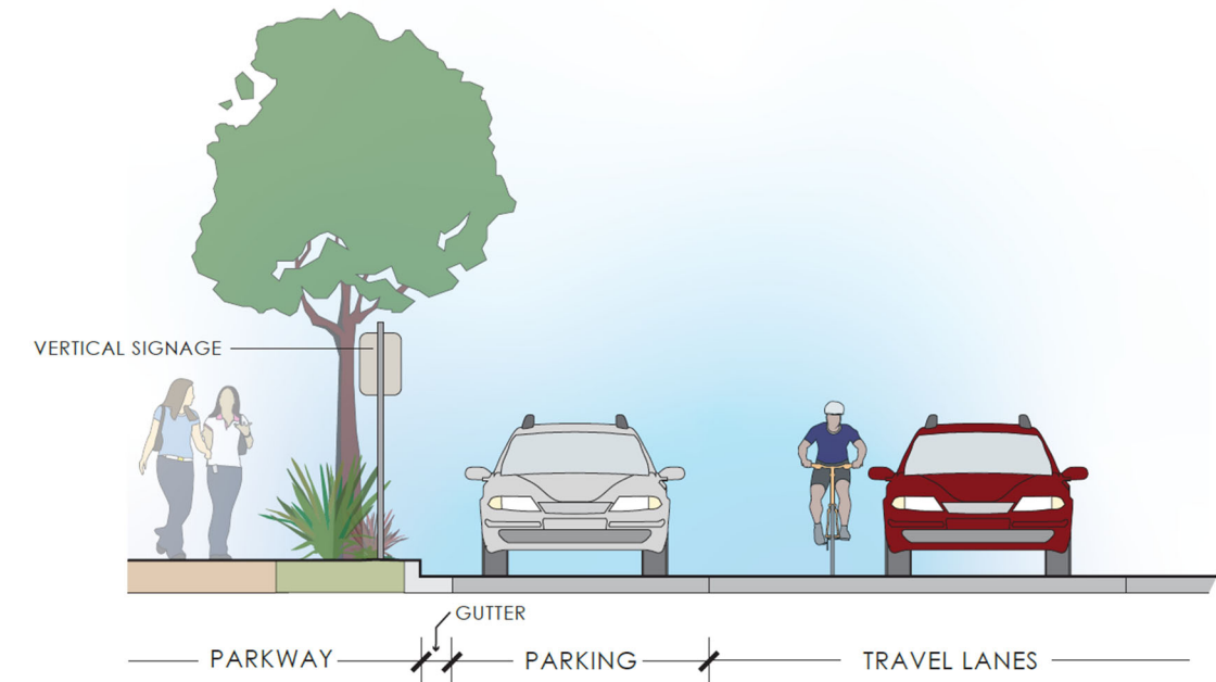
FIGURE 5-14 CLASS III BIKE ROUTE SECTION VIEW
