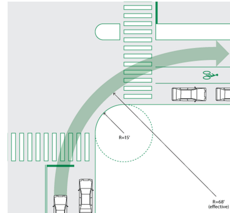
FIGURE 5-72 CURB RADIUS
