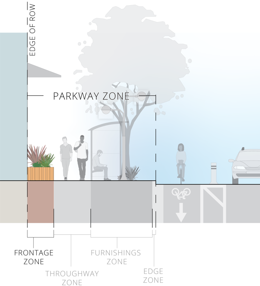
FIGURE 3-3 FRONTAGE ZONE
