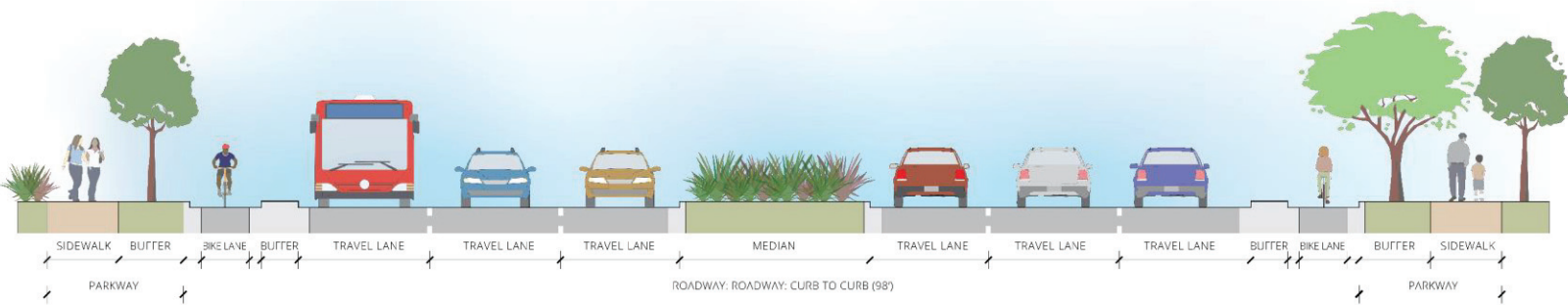
FIGURE 2-31 SIX-LANE PRIMARY ARTERIAL SECTION VIEW (OPTION C2)
