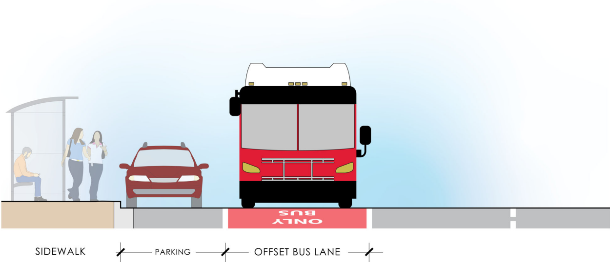
FIGURE 5-29 OFFSET BUS LANE THROUGH THE LOCATION SECTION VIEW
