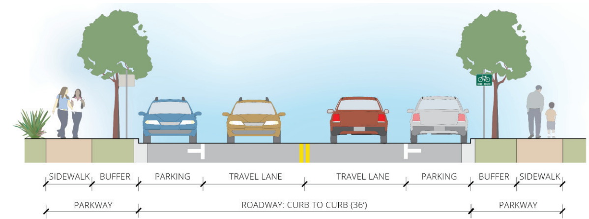
FIGURE 2-17 TWO-LANE COLLECTOR SECTION VIEW (OPTION C3)
