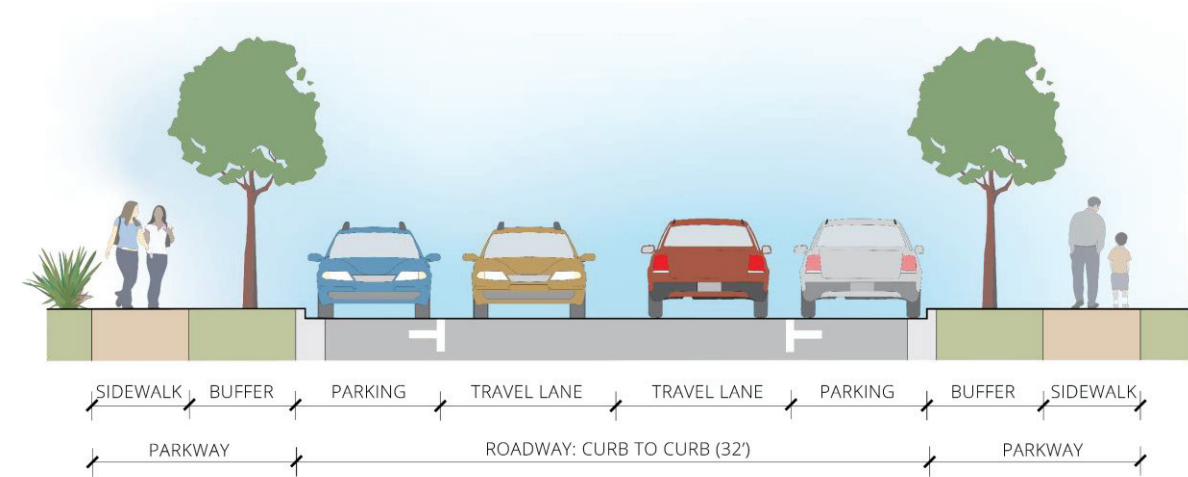
FIGURE 2-9 RESIDENTIAL LOCAL STREET SECTION VIEW (OPTION C3)
