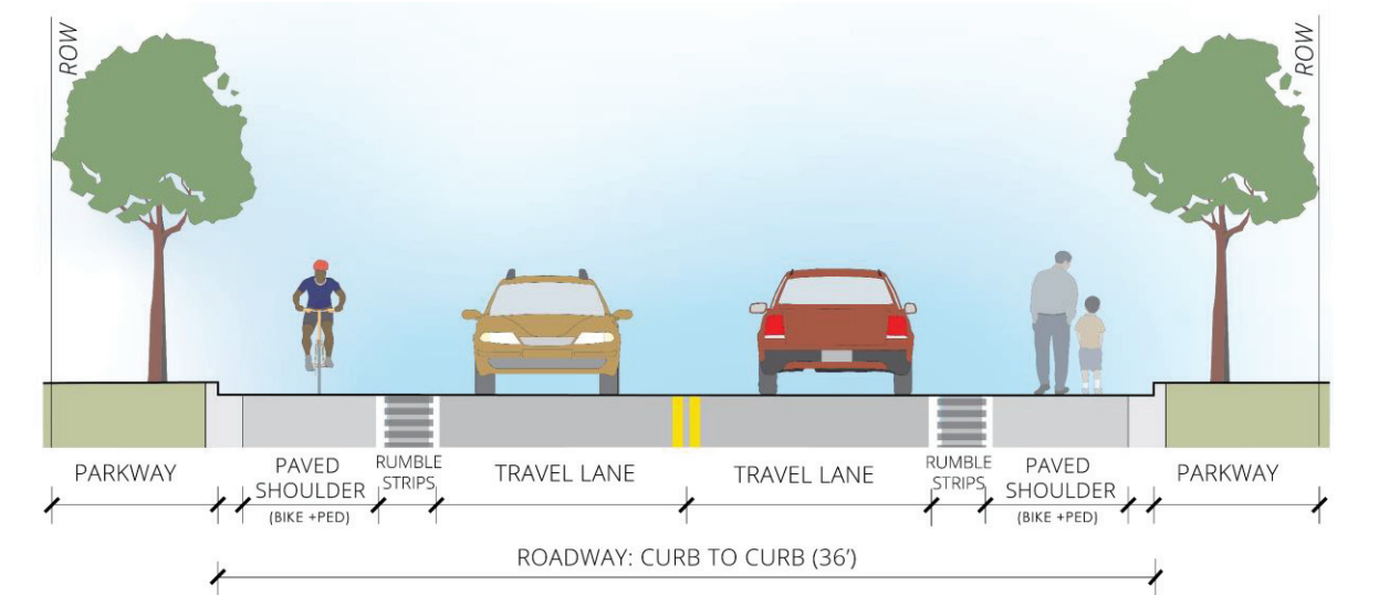
FIGURE 2-33 RURAL LOCAL ROAD SECTION VIEW (OPTION C2)
