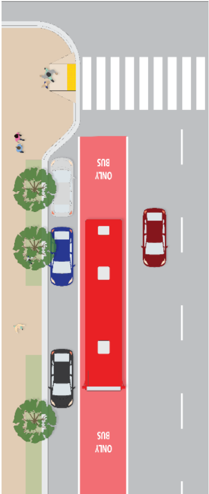
FIGURE 5-38 OFFSET BUS LANE PLAN VIEW
