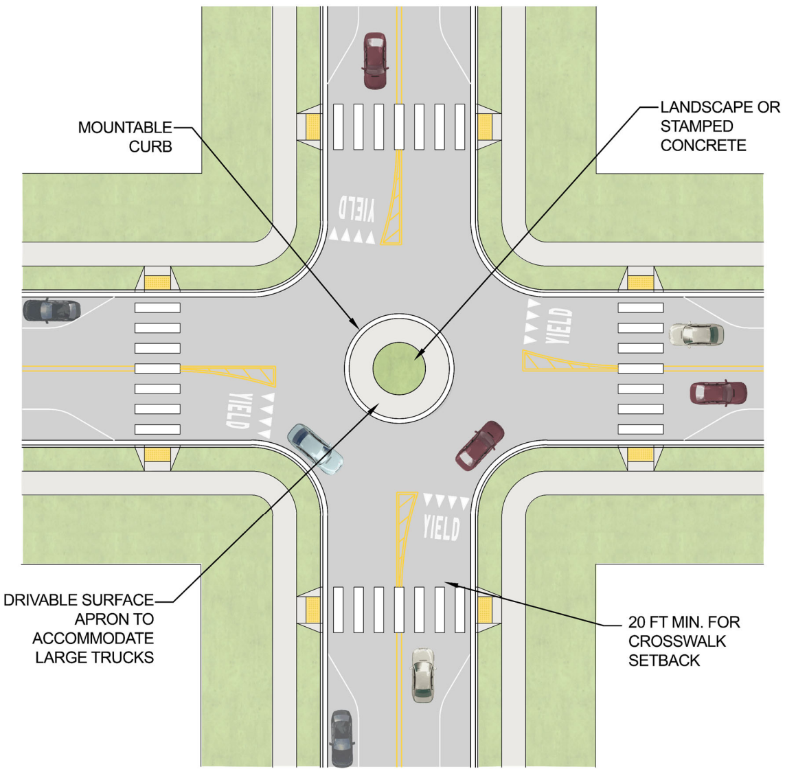
FIGURE 6-31 TRAFFIC CIRCLE
