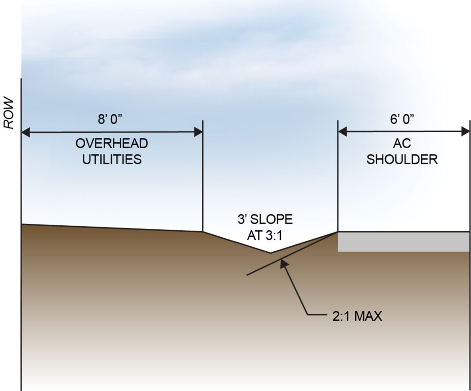
FIGURE 3-25 RP-2: 14' RURAL PARKWAY
