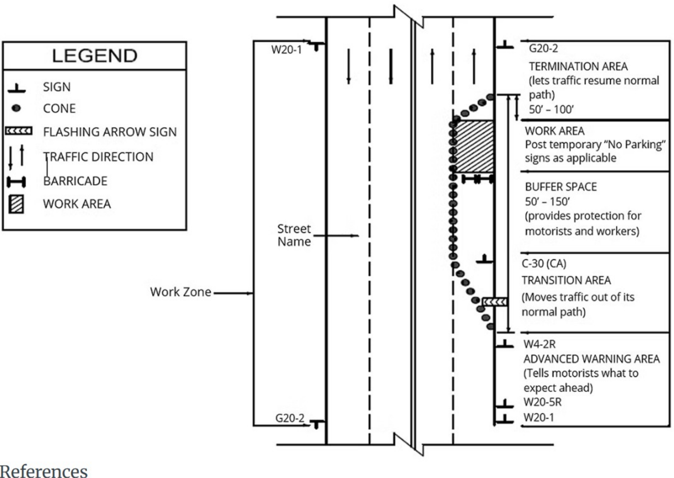
Components of a Typical Traffic Control Plan
