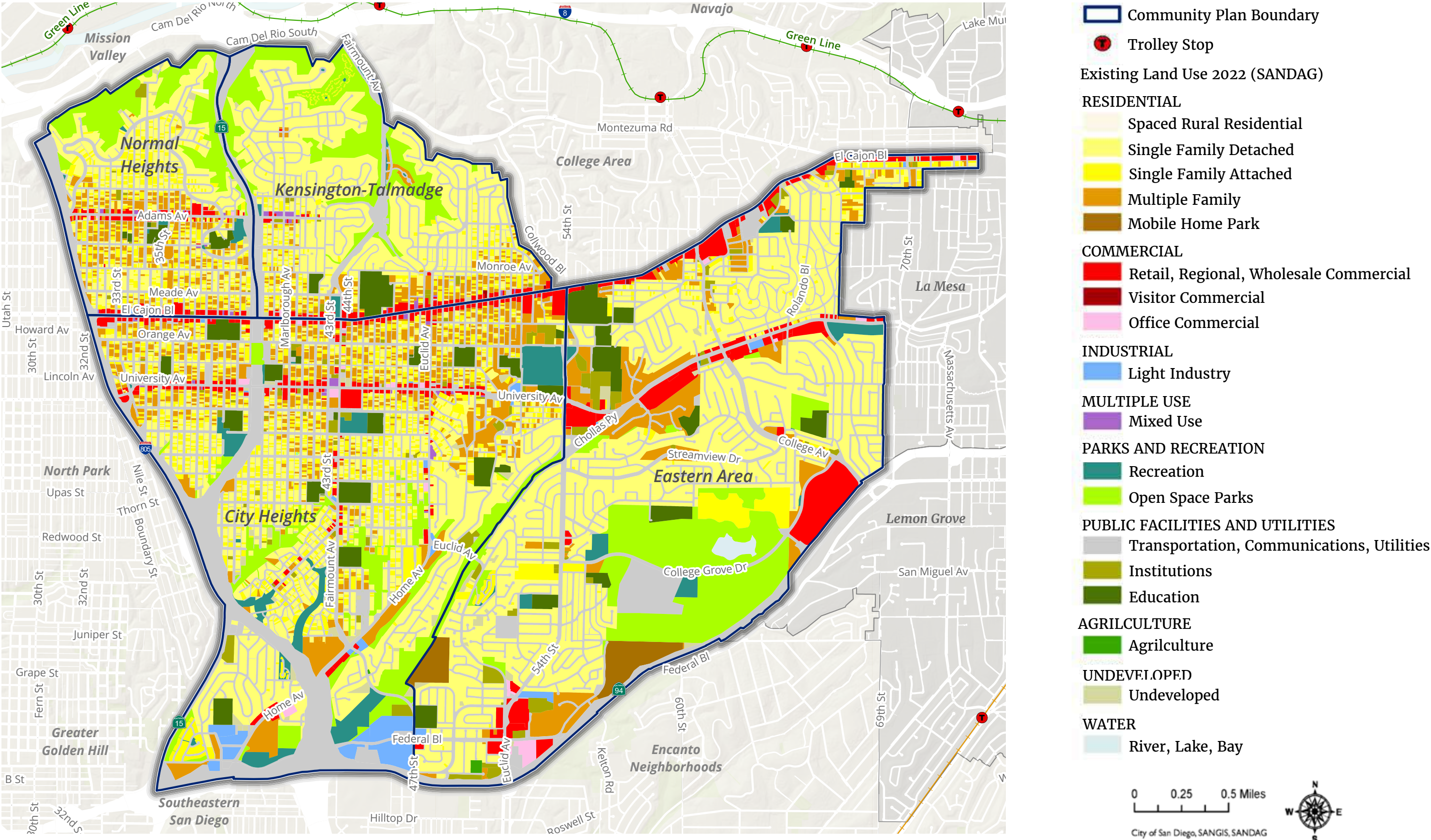
Figure 4-2 Existing Land Use
