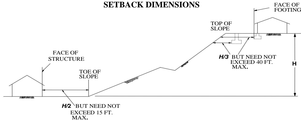
FIGURE 3 SETBACK DIMENSIONS
