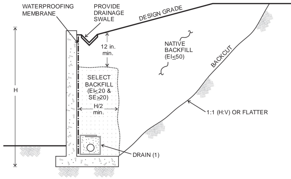
Detail RTW-A
