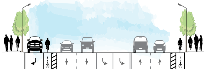
Figure 3-10 Garnet Avenue/Balboa Avenue Between Santa Fe Street and Moraga Avenue
