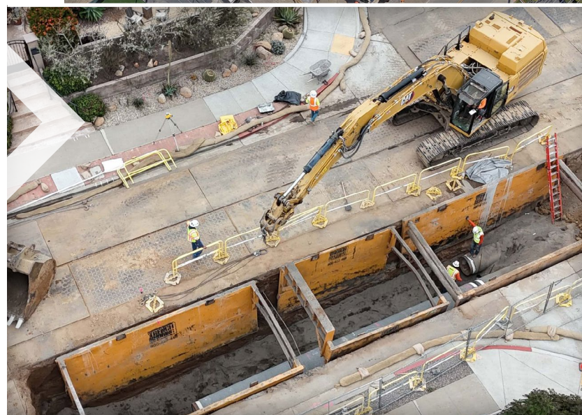
Morena Conveyance South & Middle Alignment
