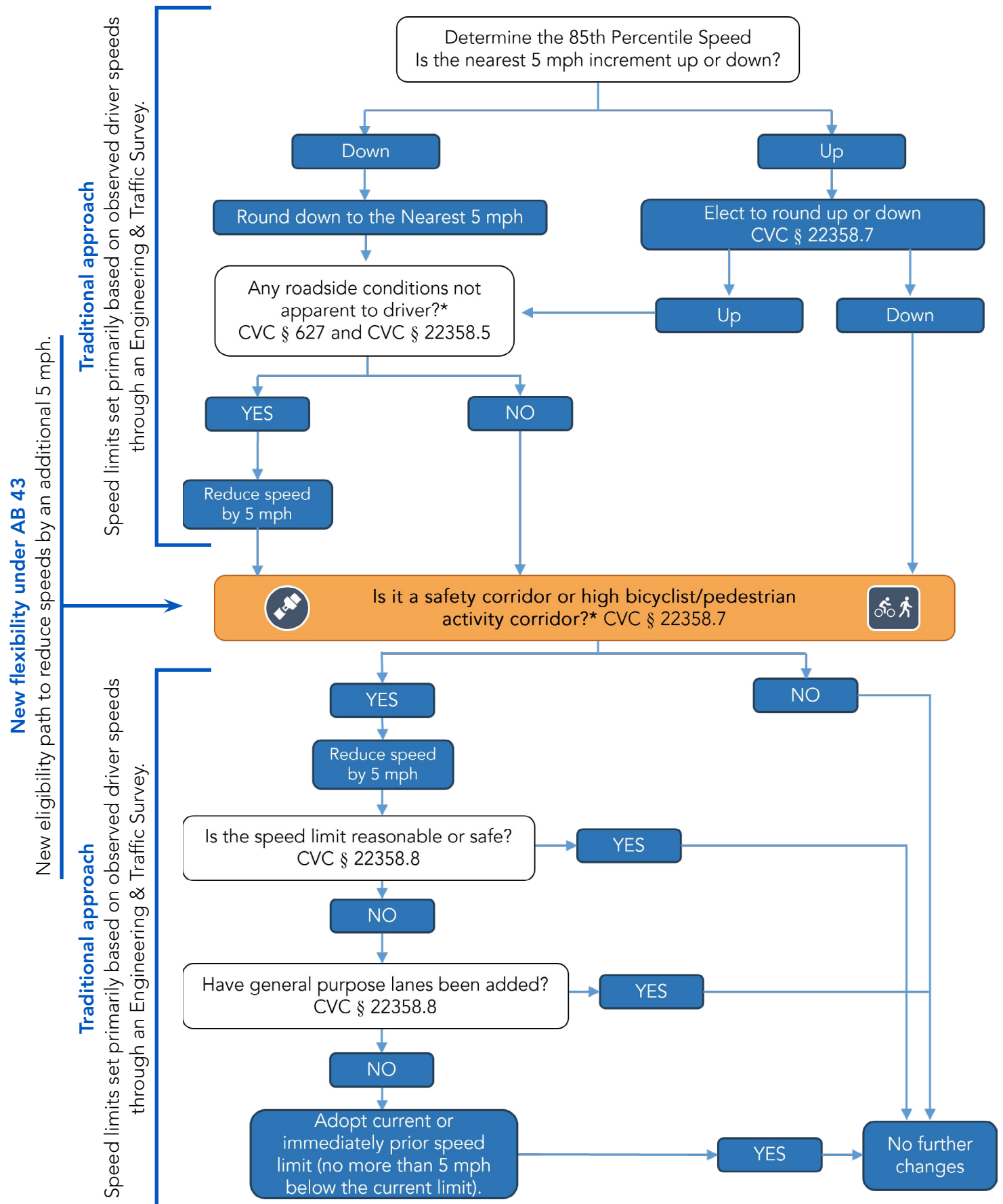
Figure 1 | General Process for Establishing Speed Limits Through an E&TS
