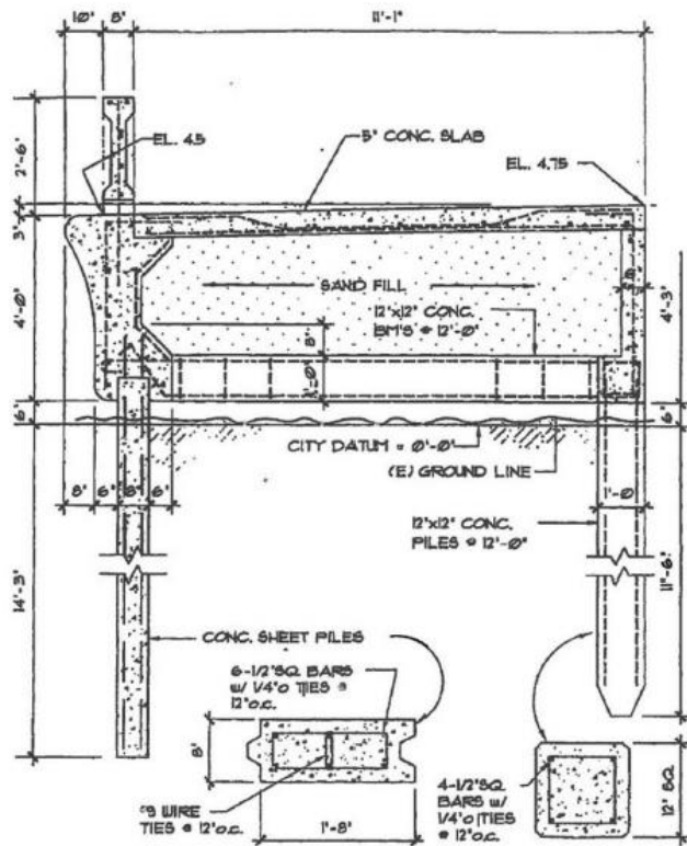
Figure 3-1. 1925 Seawall Section
