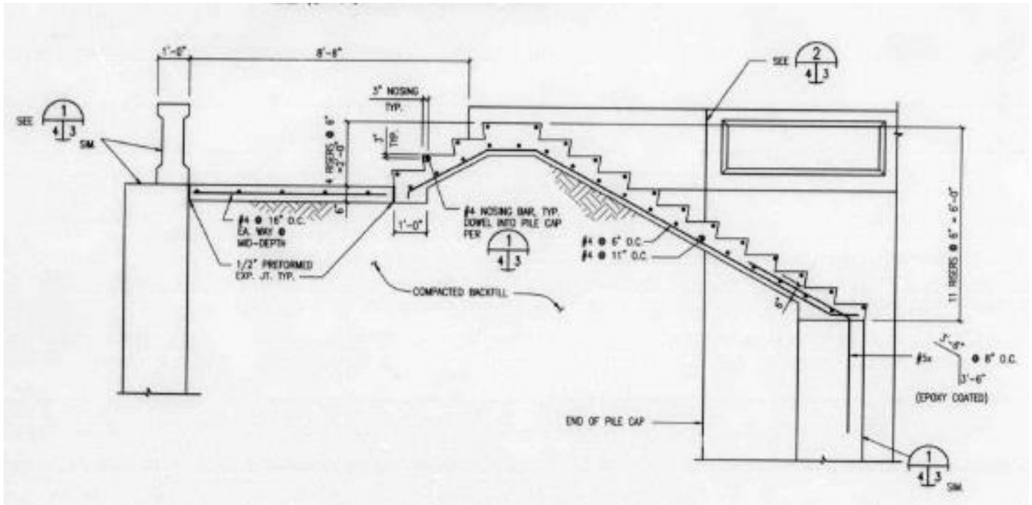
Figure 4-8. Existing Stair Example (1999 plans)
