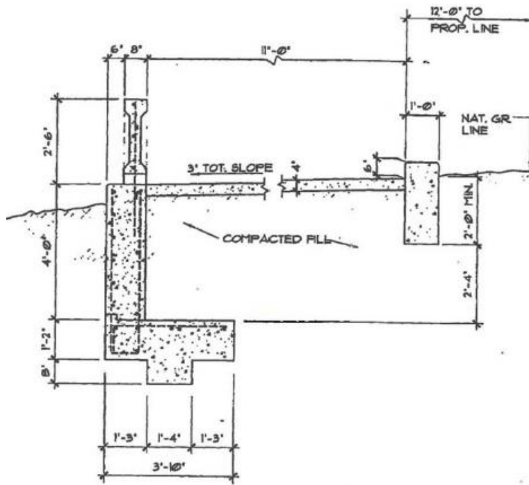
Figure 3-3. 1968 Seawall Section
