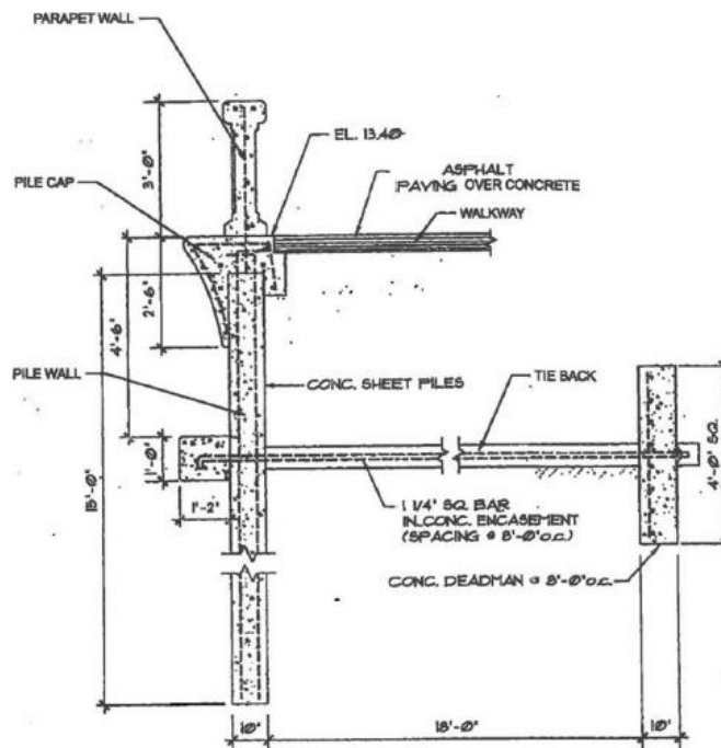
Figure 3-2. 1928 Seawall Section
