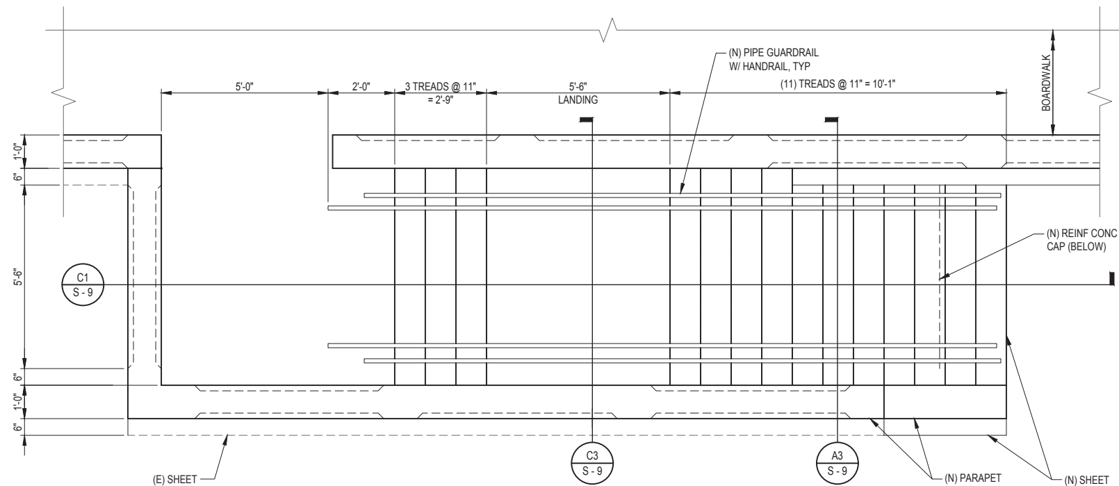
BEACH ACCESS STAIR PLAN SCALE: 1/2" = 1'-0"
