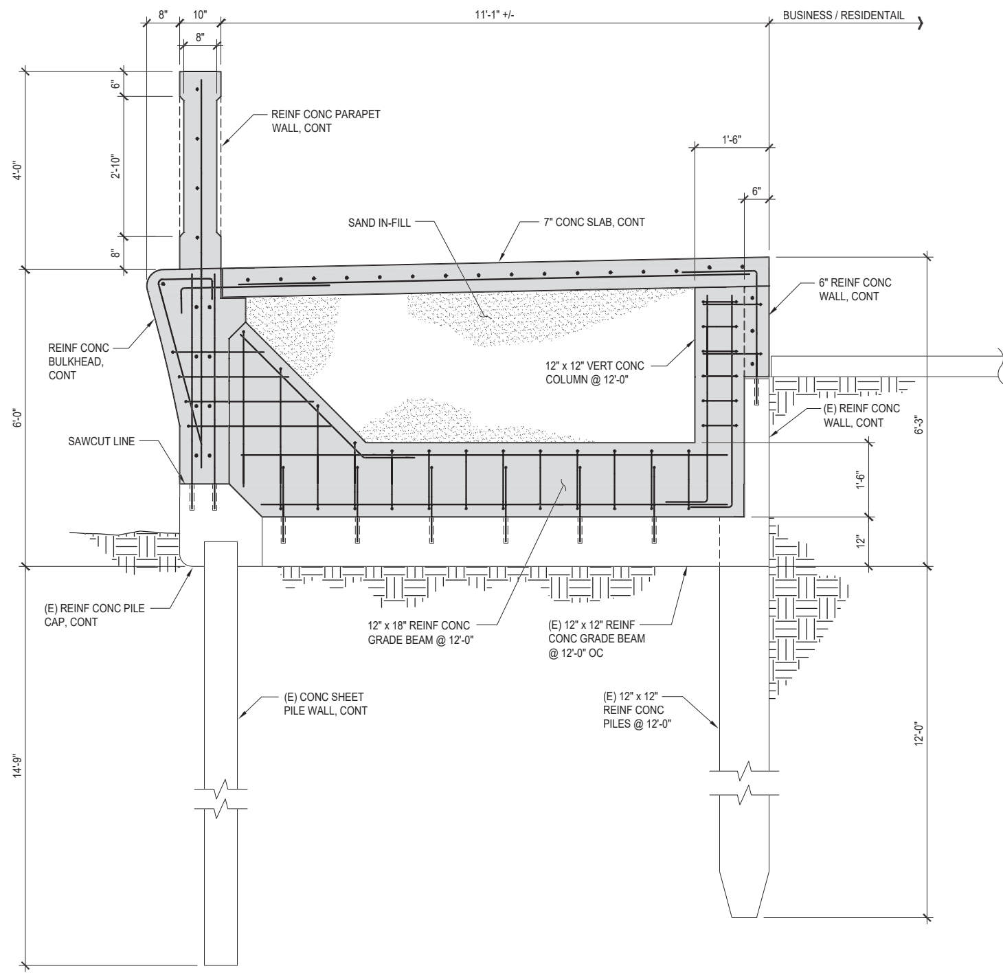
SEGMENT A - OPTION 2: RAISED BOARDWALK 3/4" = 1'-0" STA 1+00.00 TO STA 19+85.00 STA 100+00.00 TO STA 167.73.33
