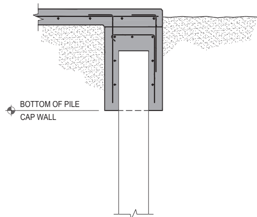
DETAIL 1/2" = 1'-0"
