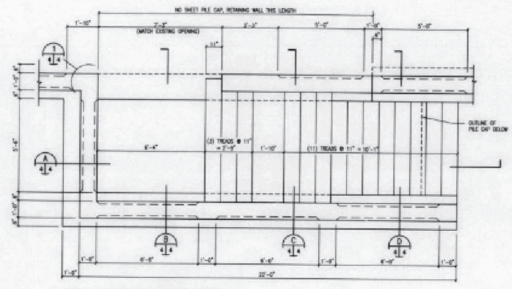
STAIR PLAN (TYP. OF (2)) SCALE: 1/2" = 1'-0"
