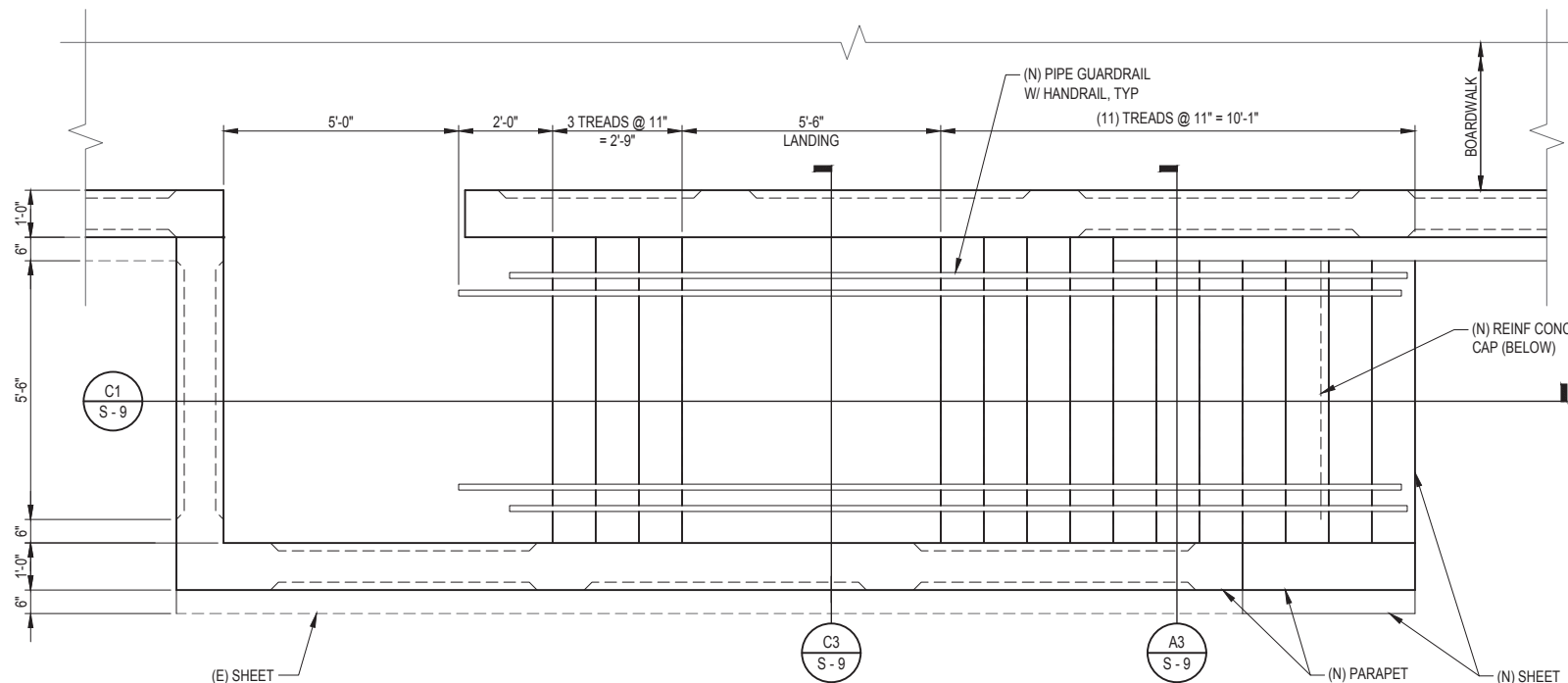
BEACH ACCESS STAIR PLAN
