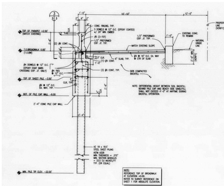
Figure 3-4. 2000 Seawall Section
