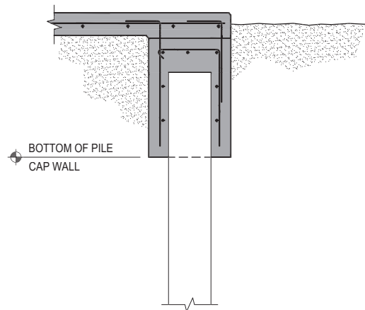
DETAIL 1/2" = 1'-0"
