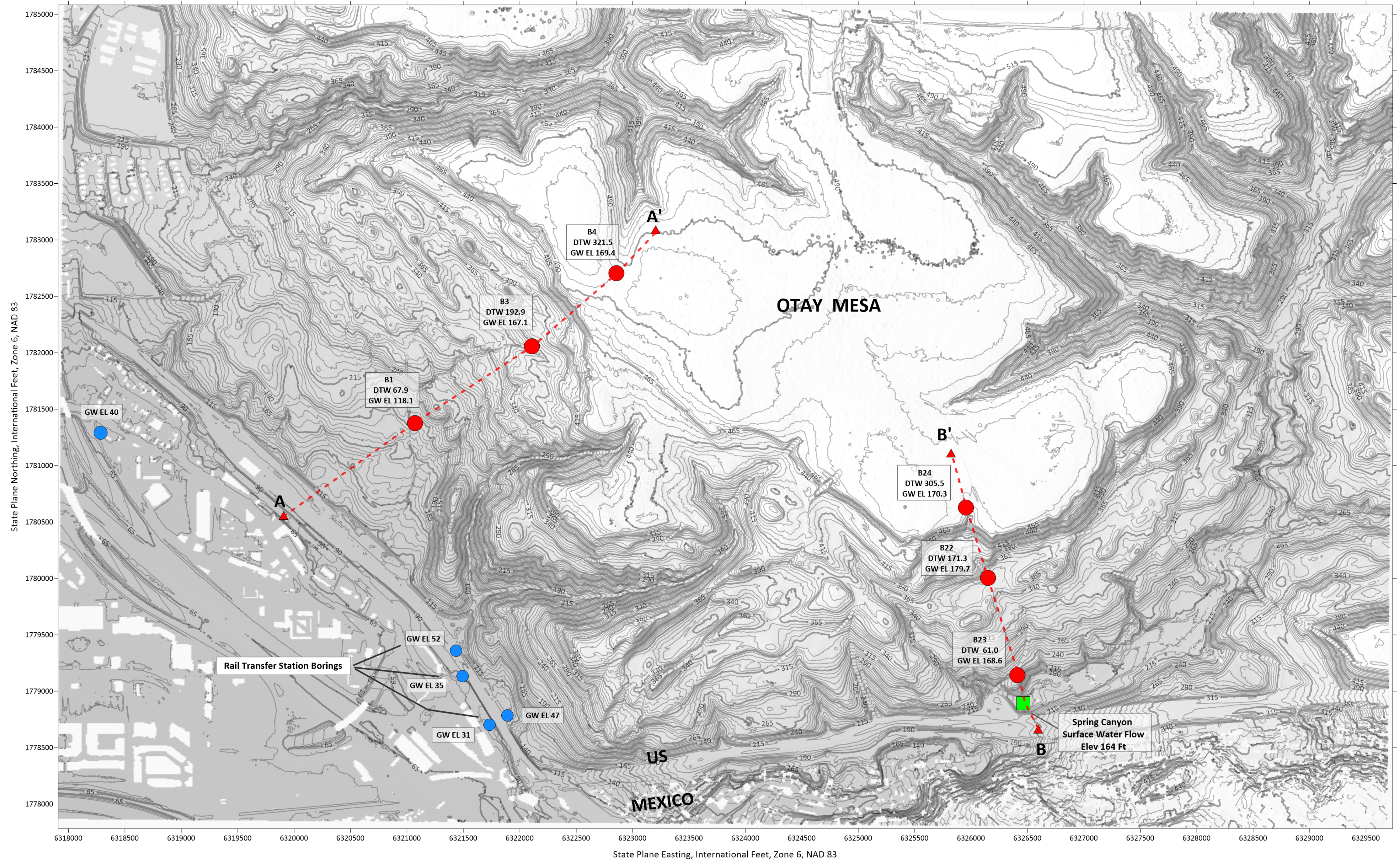
FIGURE 2, Revised Shaded Relief Topographic Map Showing Geocon Landslide Investigation Coreholes and Monitor Well Locations Otay Mesa, San Diego County, CA
