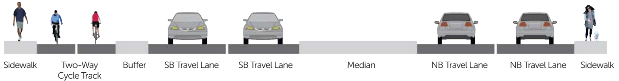
Figure 3-7 - Proposed Cross Section for Improvement 5
