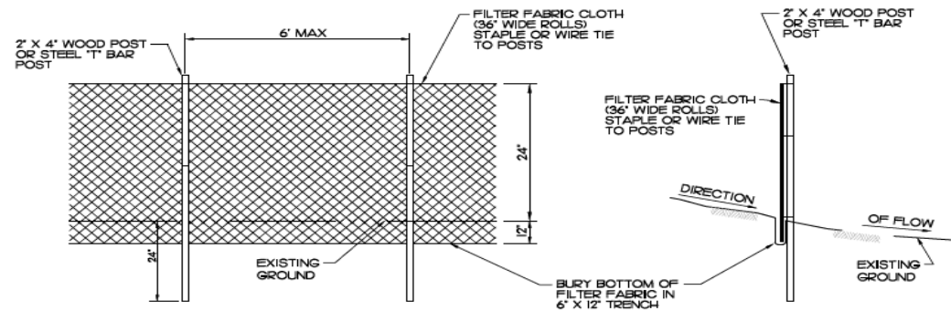
A SILT FENCE DETAIL NO SCALE
