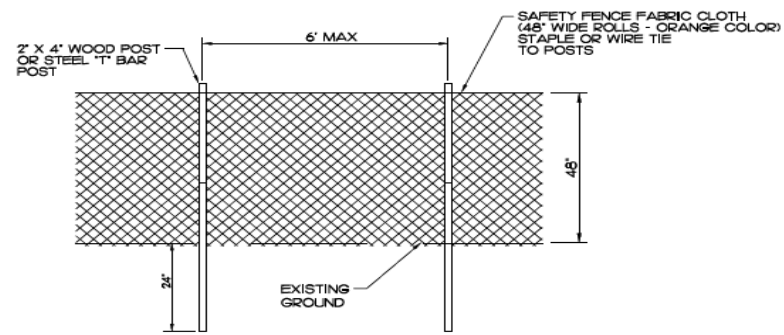
B OSHA FENCE DETAIL NO SCALE
