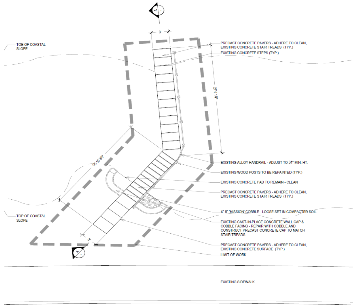
REPAIR PLAN
