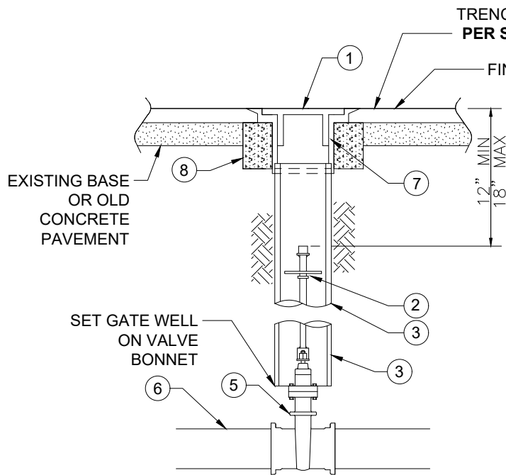
GATE WELLS (GATE VALVES)
