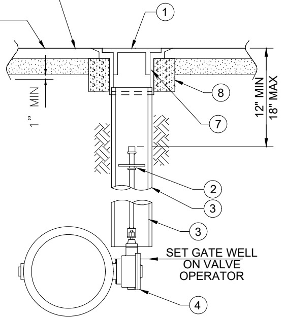
GATE WELLS (BUTTERFLY VALVES)
