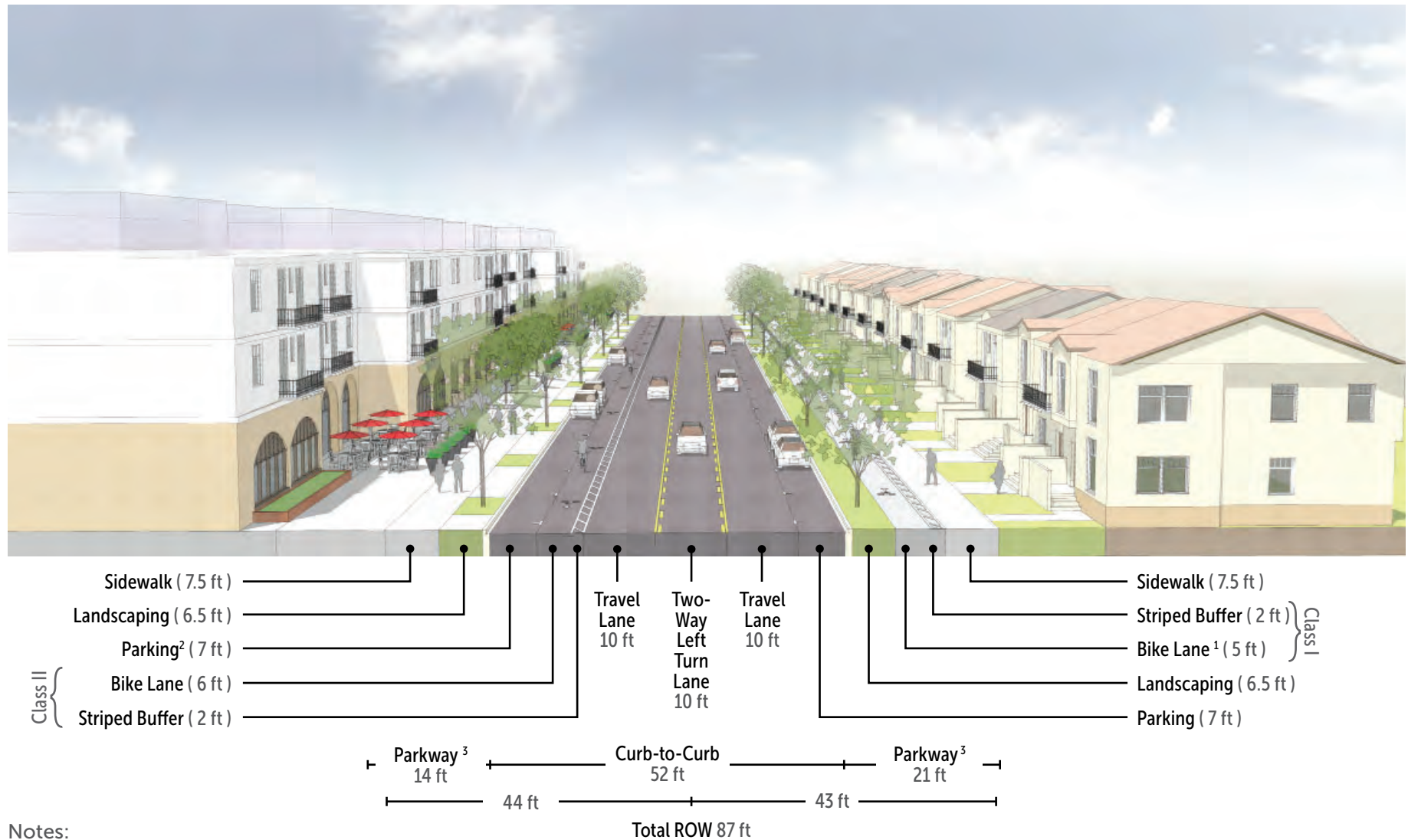
Figure 4.11 — Modified Cross-Section for 2-Lane Collector with Two-Way Center Left Turn Lane, Class II Bike Lane with Buffer on West Side, and Class I Bike Path on East Side
