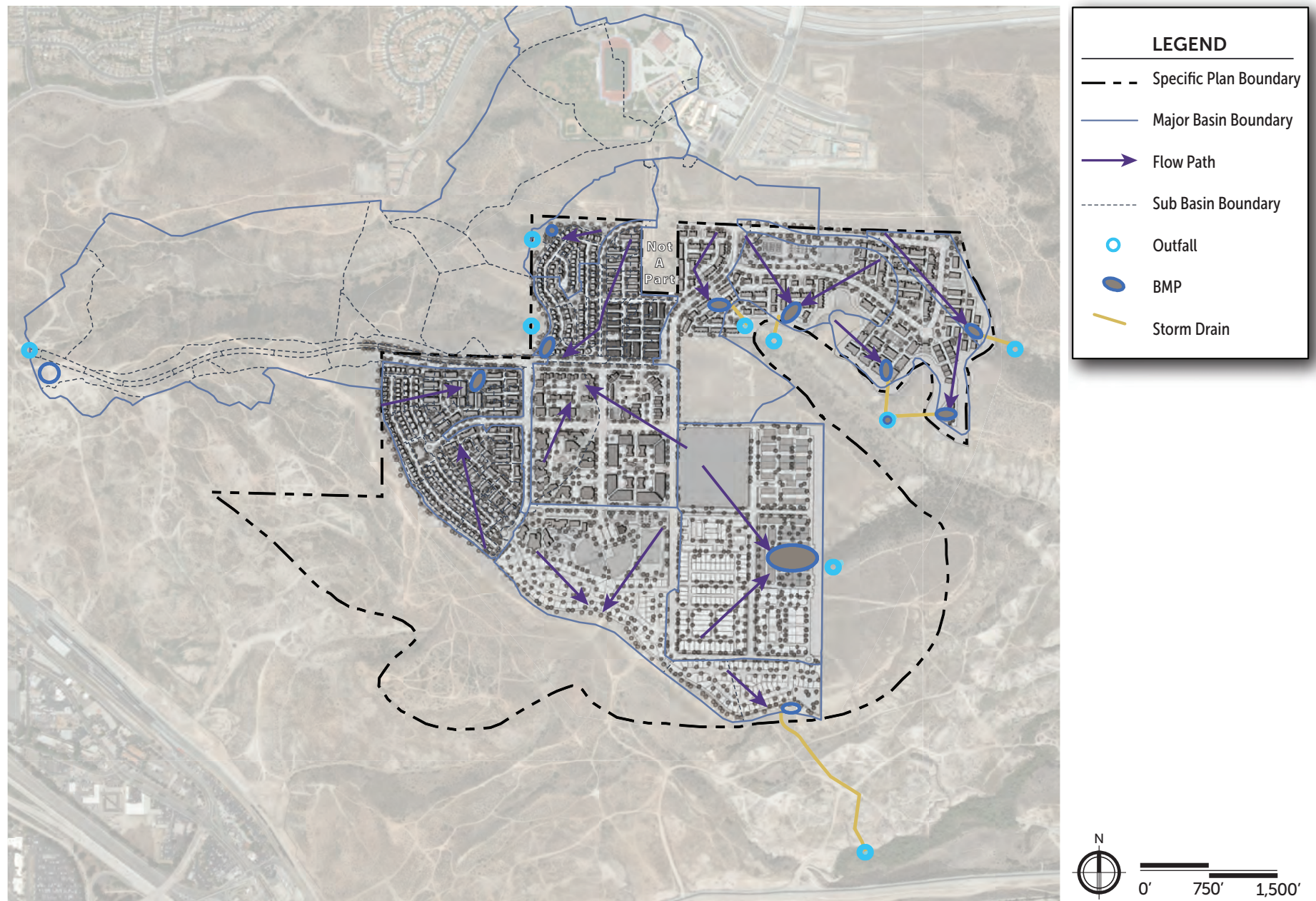
Figure 6.3 — Drainage System
