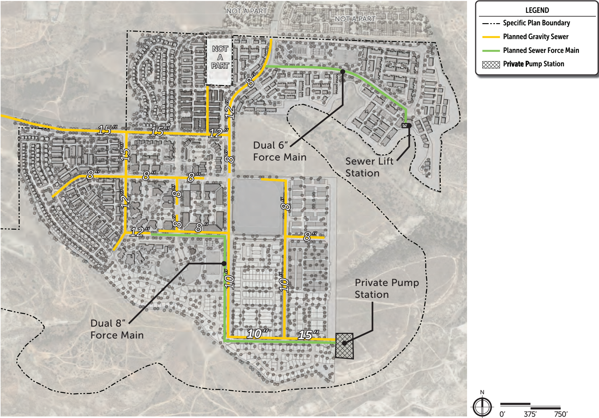
Figure 6.2 – Sewer System within the Specific Plan Area
