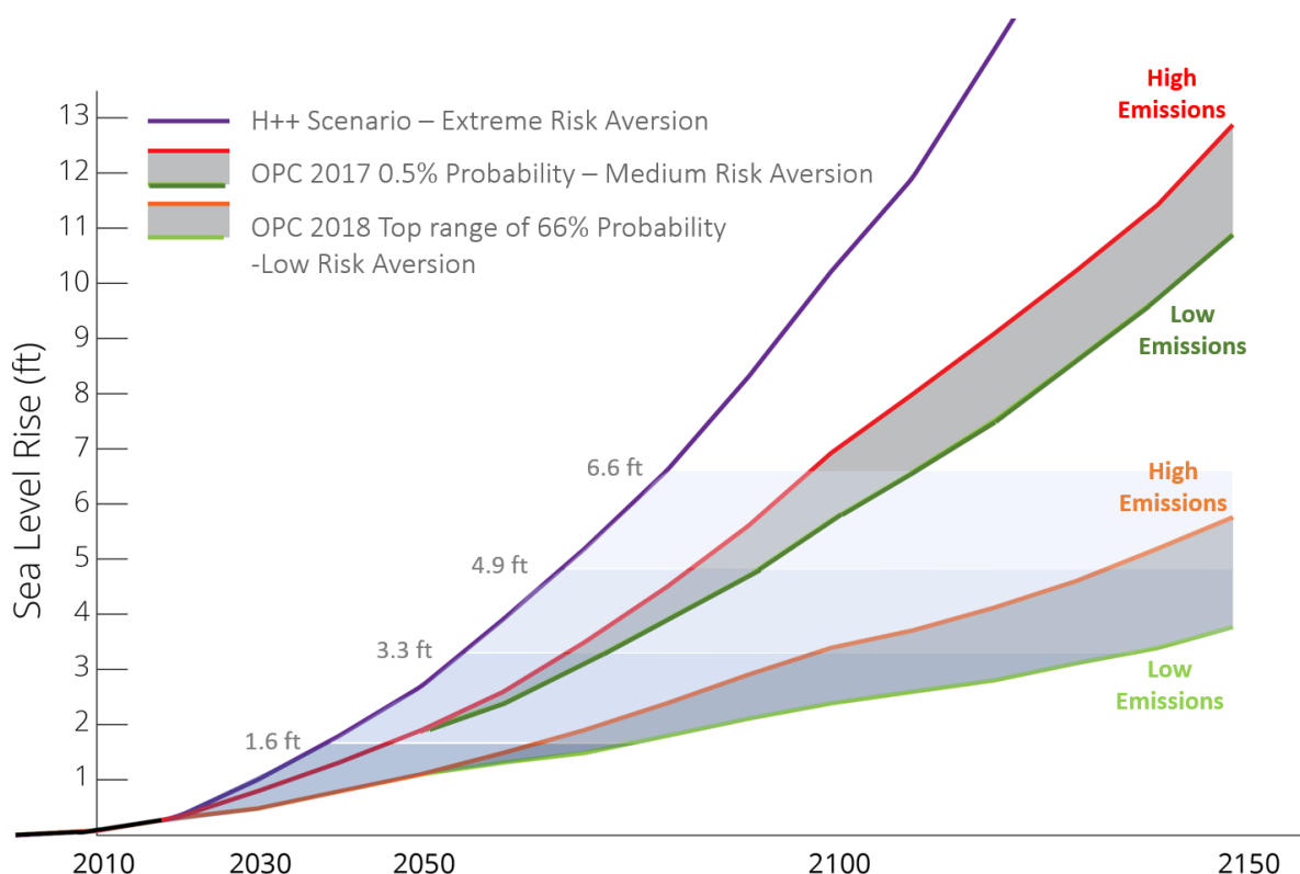
Figure 3 Likely ranges of sea level rise from OPC (2018)
