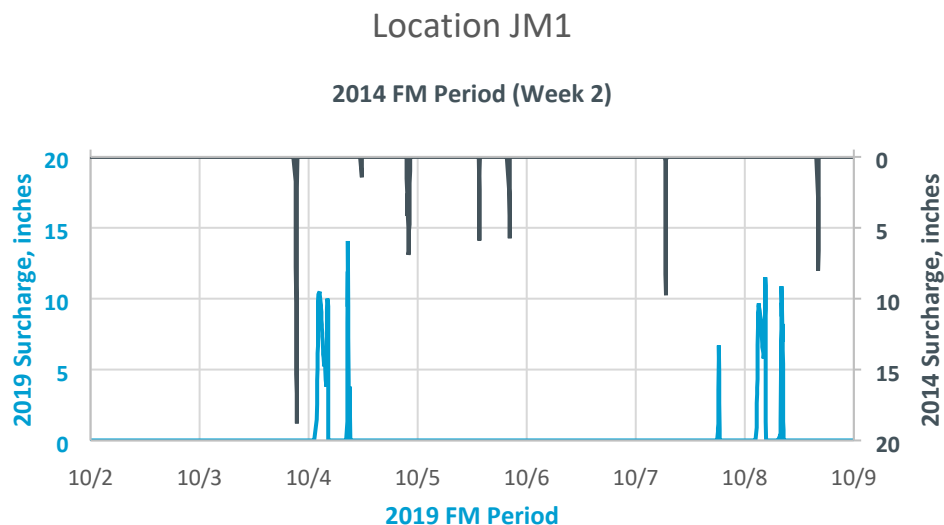
Figure 2 . Comparison of Surcharges at Location JM1
