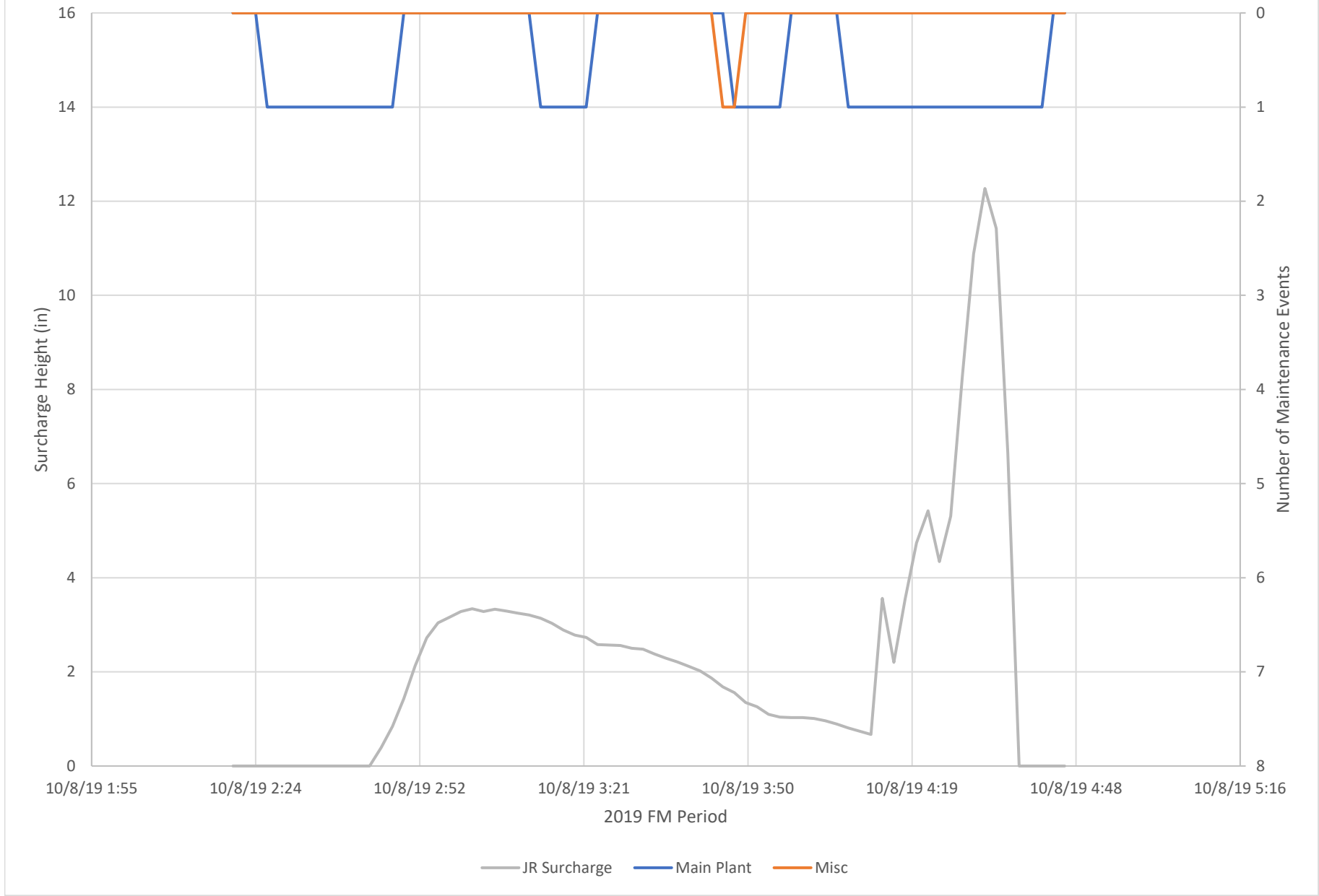
JR - Surcharge Event 3
