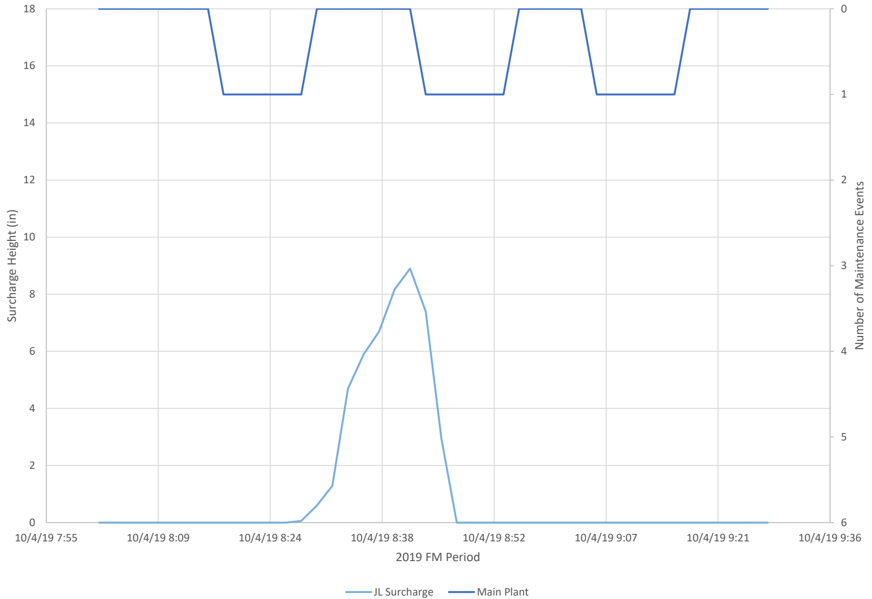
JL - Surcharge Event 1
