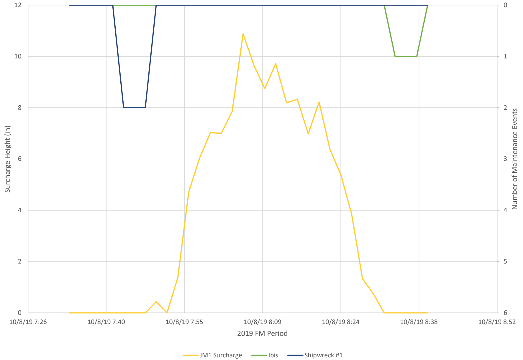
JM1 - Surcharge Event 5
