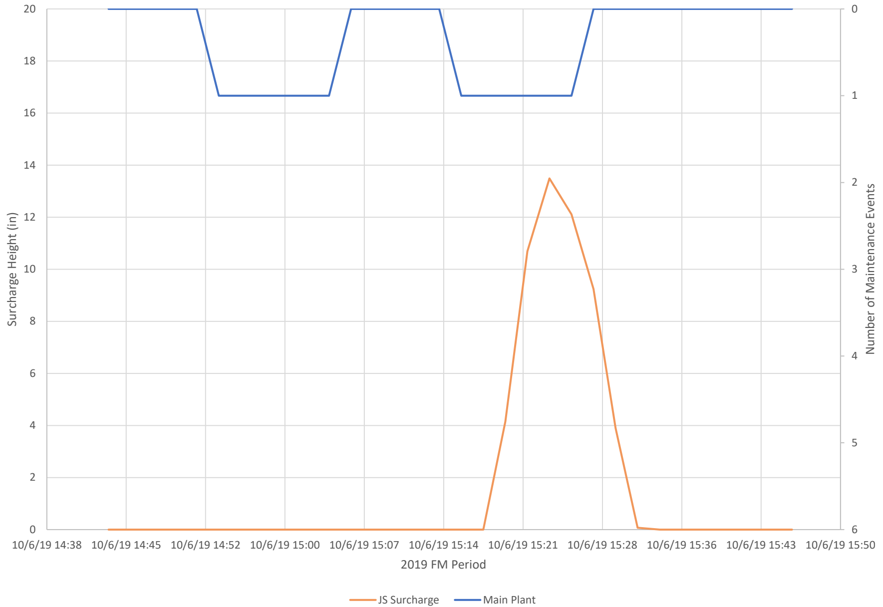
JS - Surcharge Event 6
