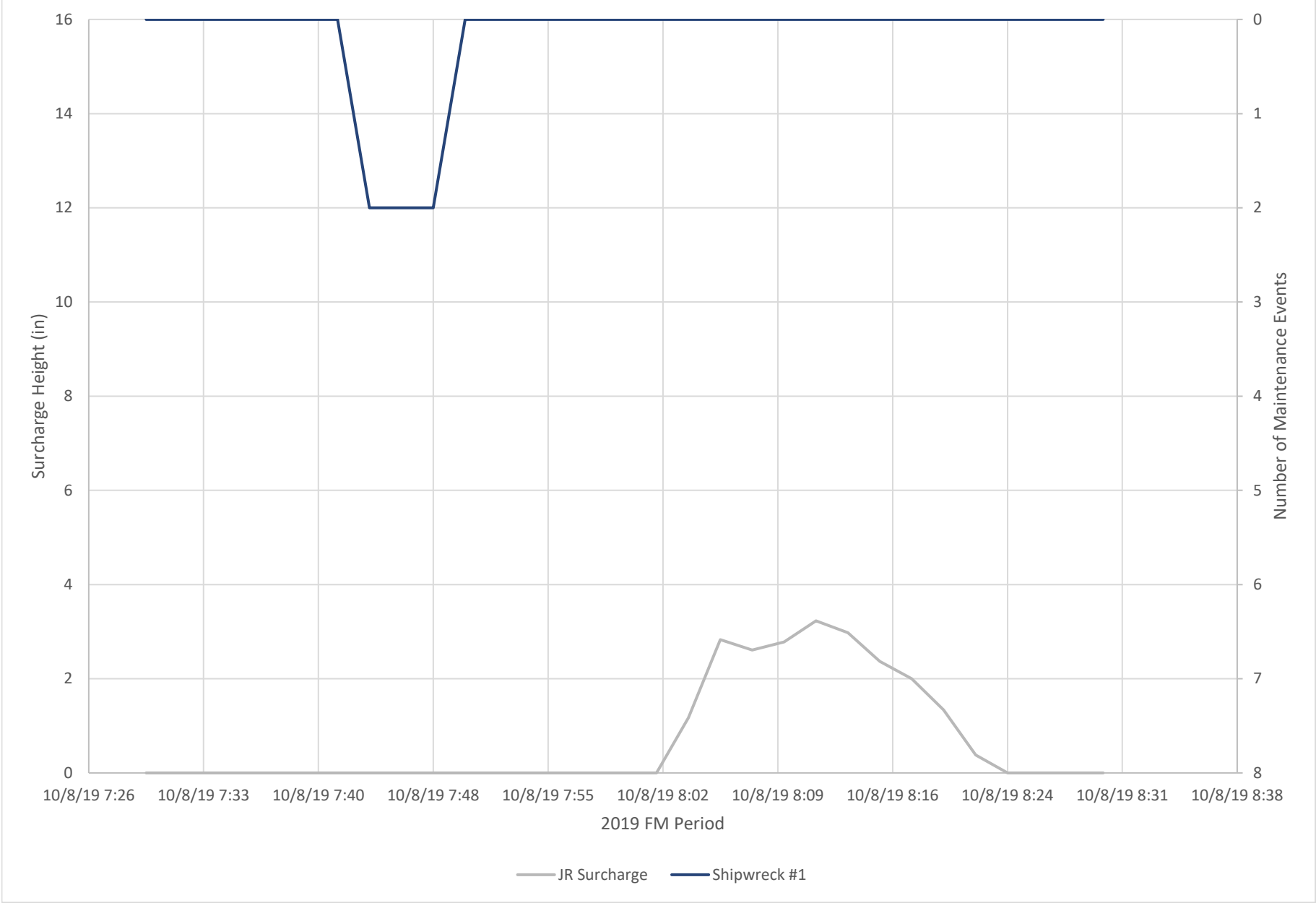
JR - Surcharge Event 4
