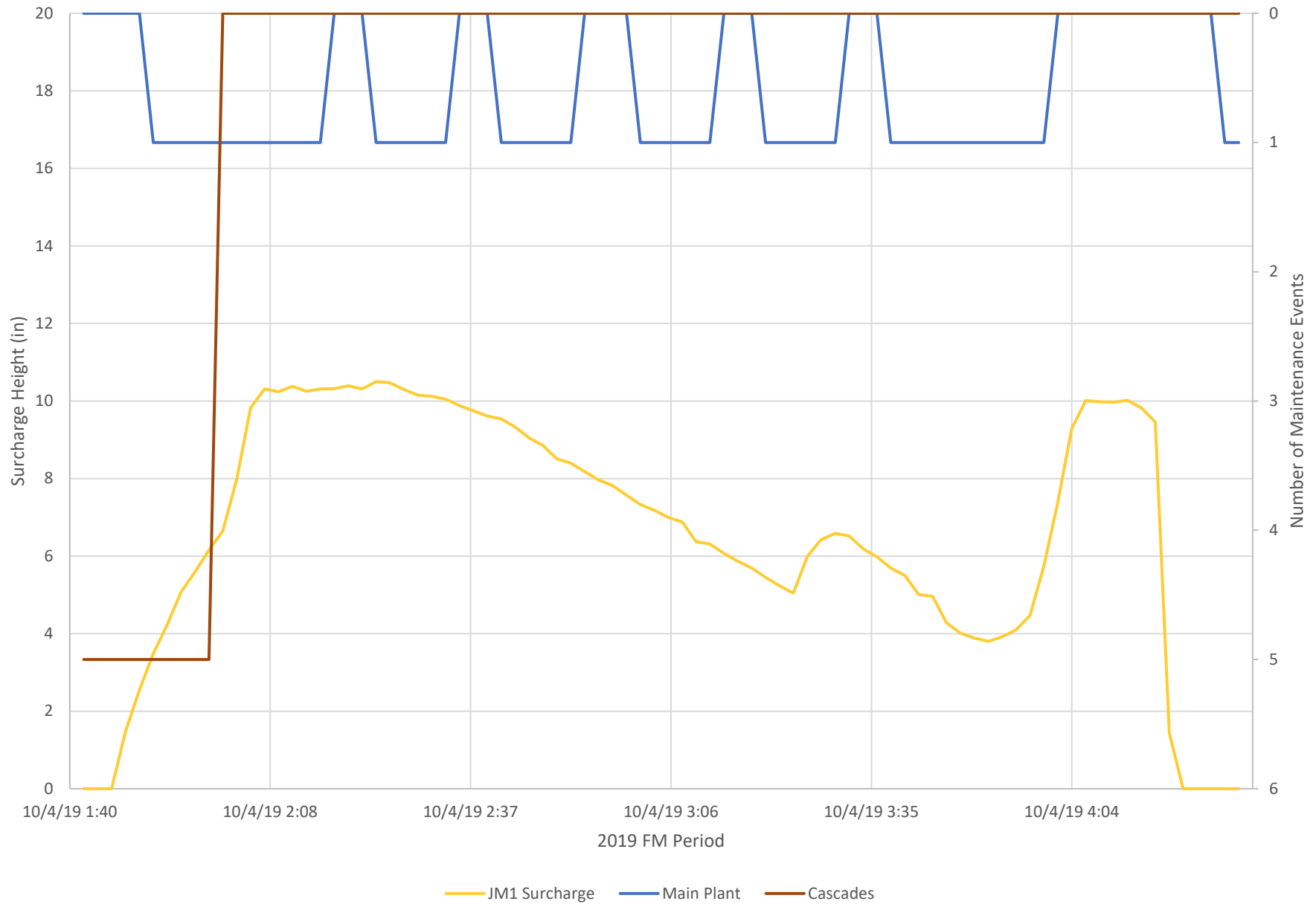
JM1 - Surcharge Event 1
