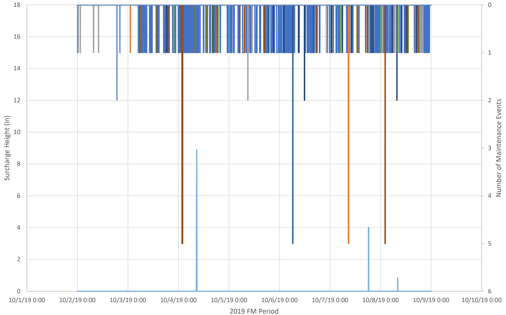
JL - Surcharge Events for 2019 Monitoring Period
