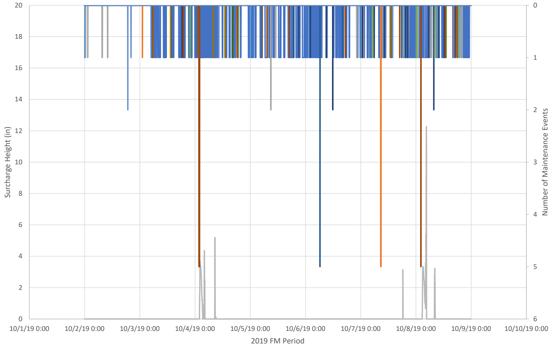
JR - Surcharge Events for 2019 Monitoring Period
