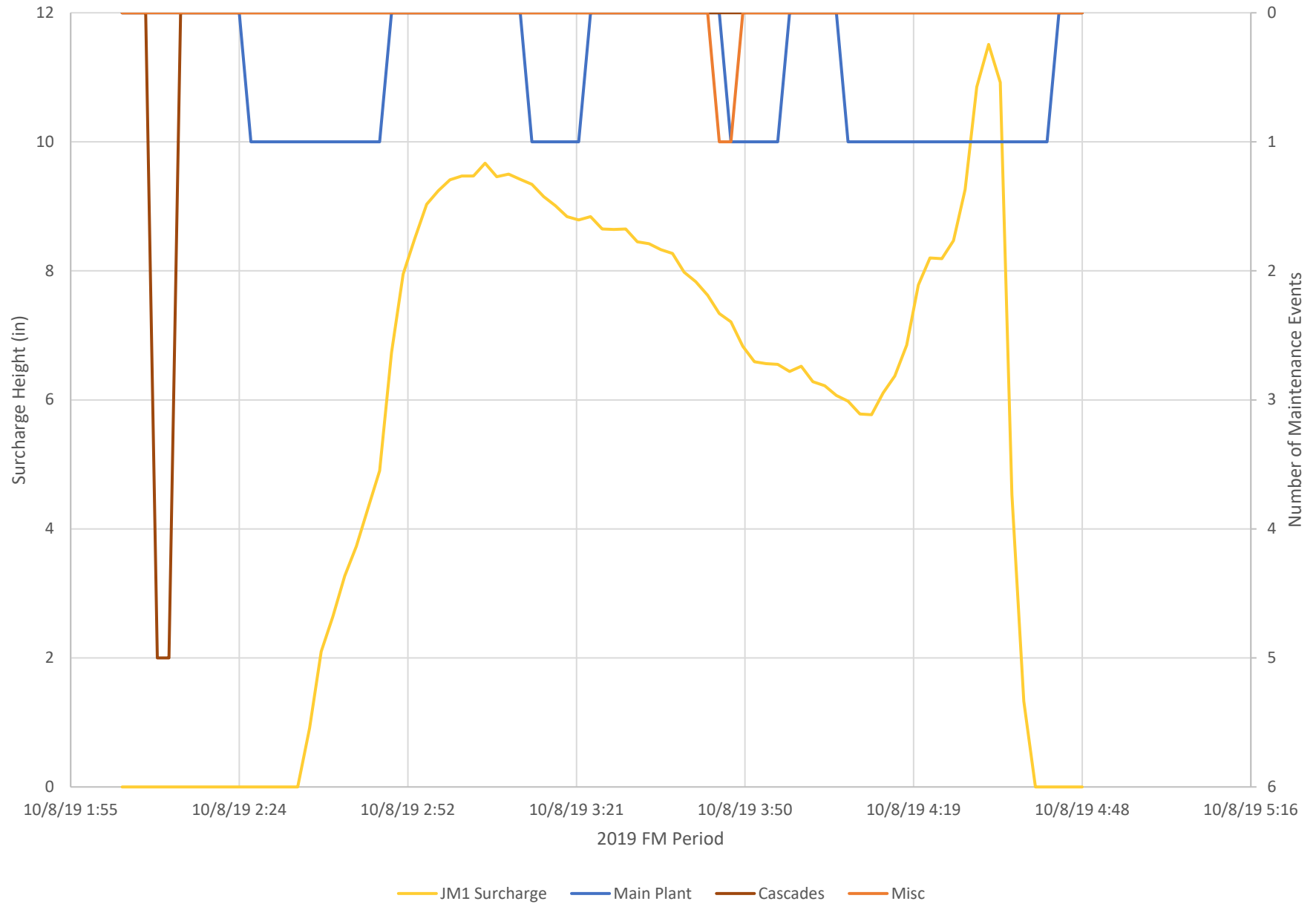
JM1 - Surcharge Event 4
