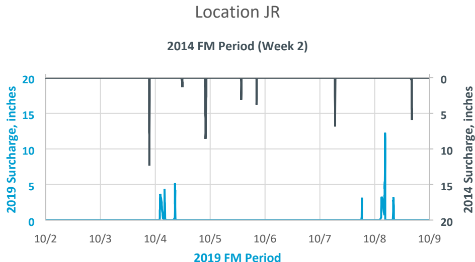
Figure 3. Comparison of Surcharges at Location JR
