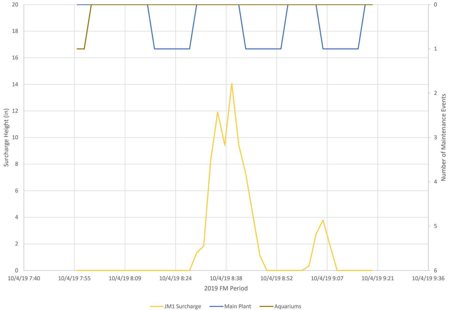
JM1 - Surge Event 2
