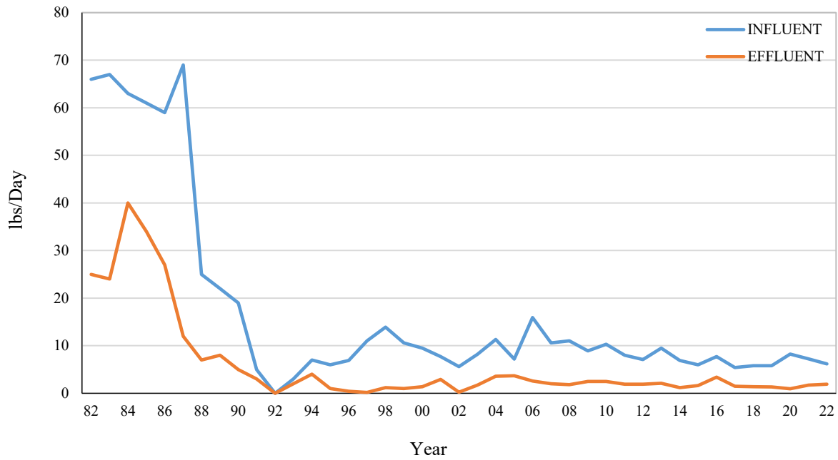
Figure 5.2-3 Chromium Point Loma Influent/Effluent History
