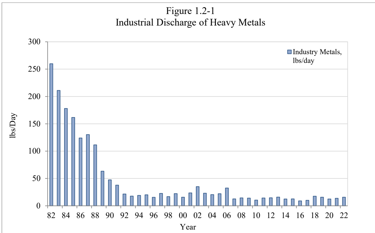
Figure 1.2-1 Average daily industrial discharge of heavy metals (cadmium, chromium, copper, lead, nickel, and zinc) to the PLWTP since IWCP approval in 1982.
