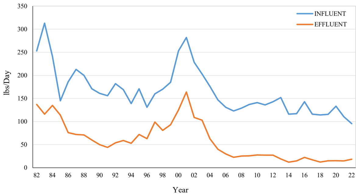
Figure 5.2-4 Copper Point Loma Influent/Effluent History
