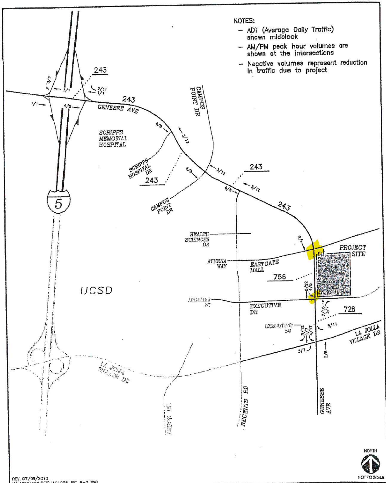
Figure 8-2 Project Traffic Volumes AM/PM Peak Hours & ADT
