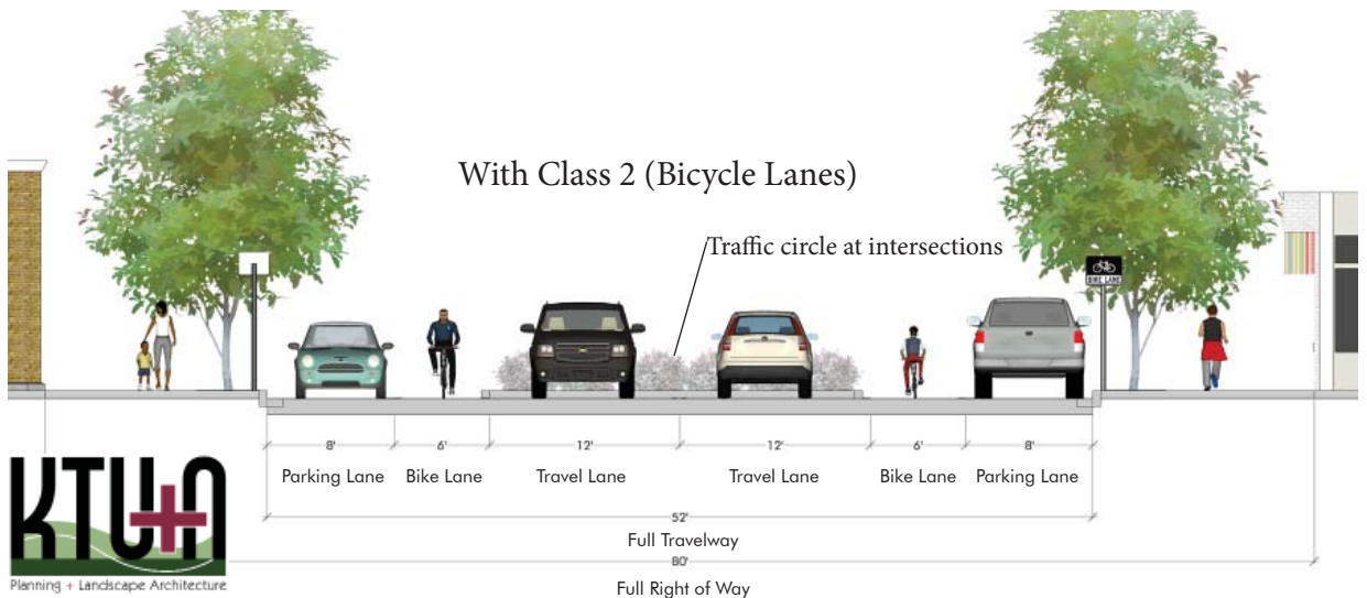
Cross-Section of 30th Street Bicycle Facility Options
