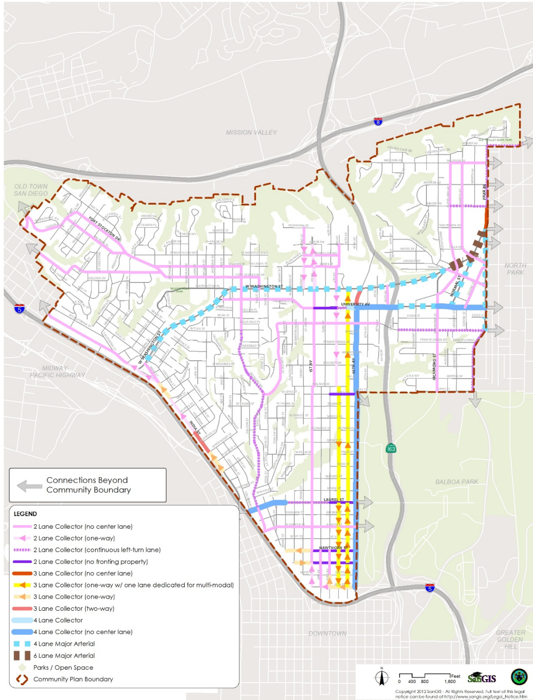
Figure 38 – Existing Functional Street Classification: Uptown
