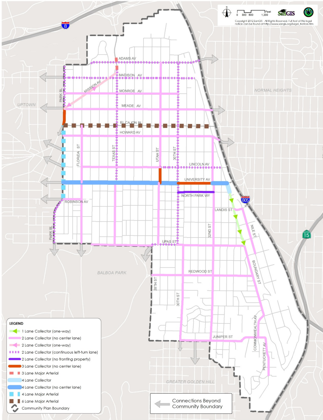
Figure 143 – Planned Street Classifications: North Park
