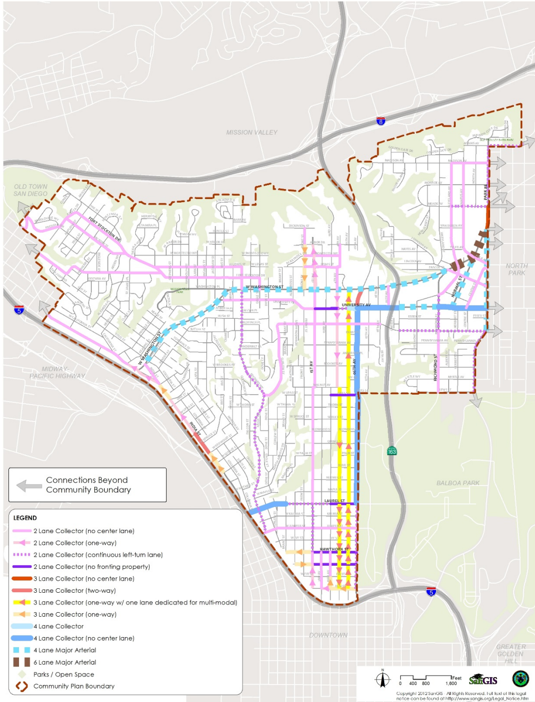
Figure 141 – Planned Street Classifications: Uptown
