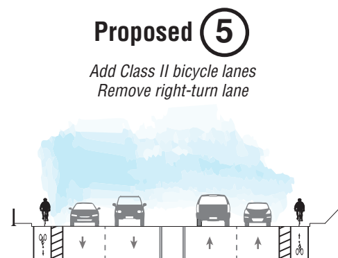
Figure 3-13 Morena Boulevard North of Ramps
