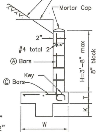
TYPICAL SECTION
