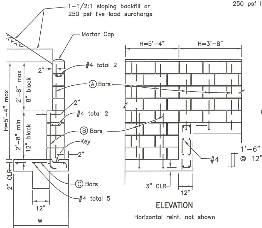
TYPICAL SECTION
