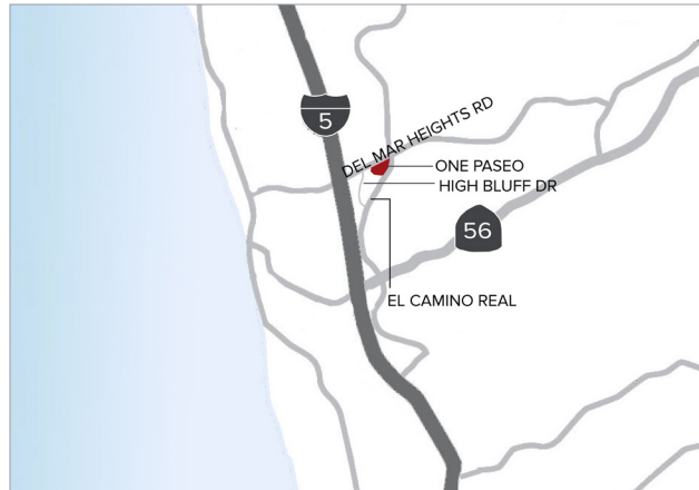
Figure 1.10a Regional Circulation
