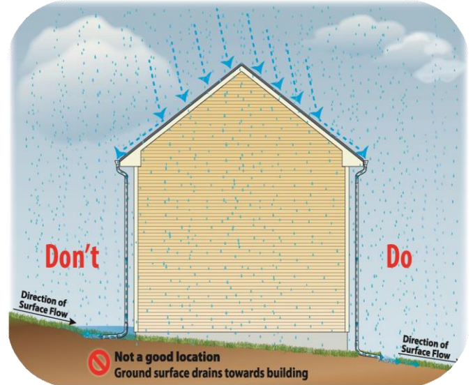
Figure 1-2. Siting Considerations
