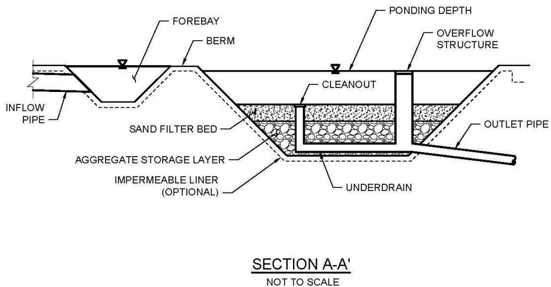
Figure E.23-1 : Typical Plan and Section View of a Sand Filter BMP
