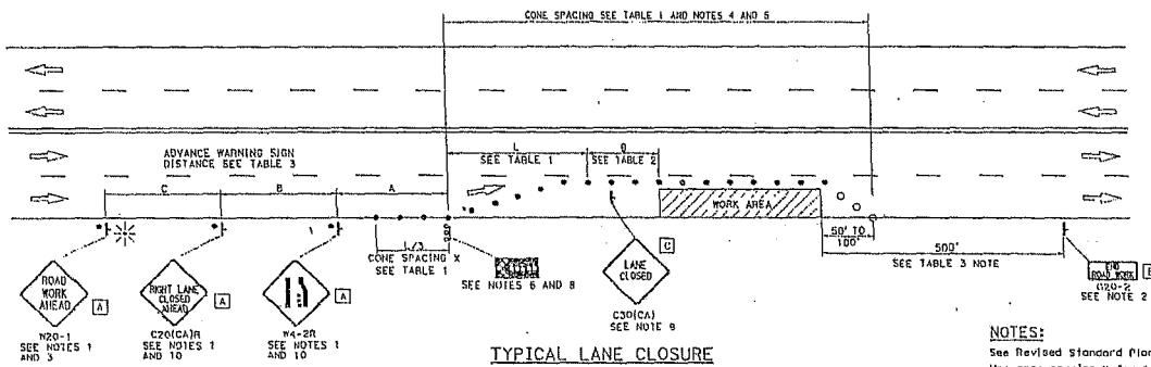
TYPICAL LANE CLOSURE
