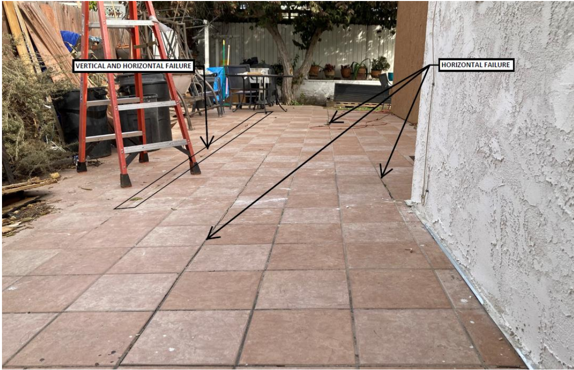
SURFACE IMPROVEMENT FAILURE AT 4310 EBERSOLE DRIVE
