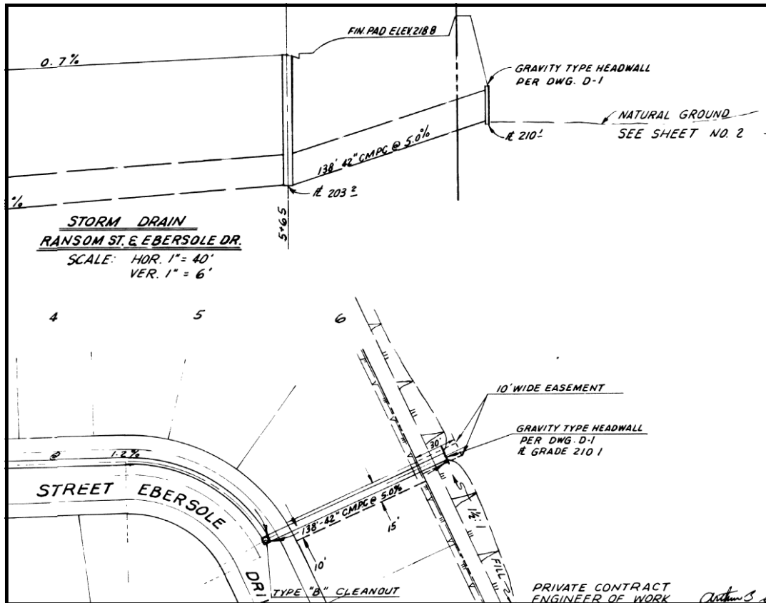
AS-BUILT 14018-12-D
