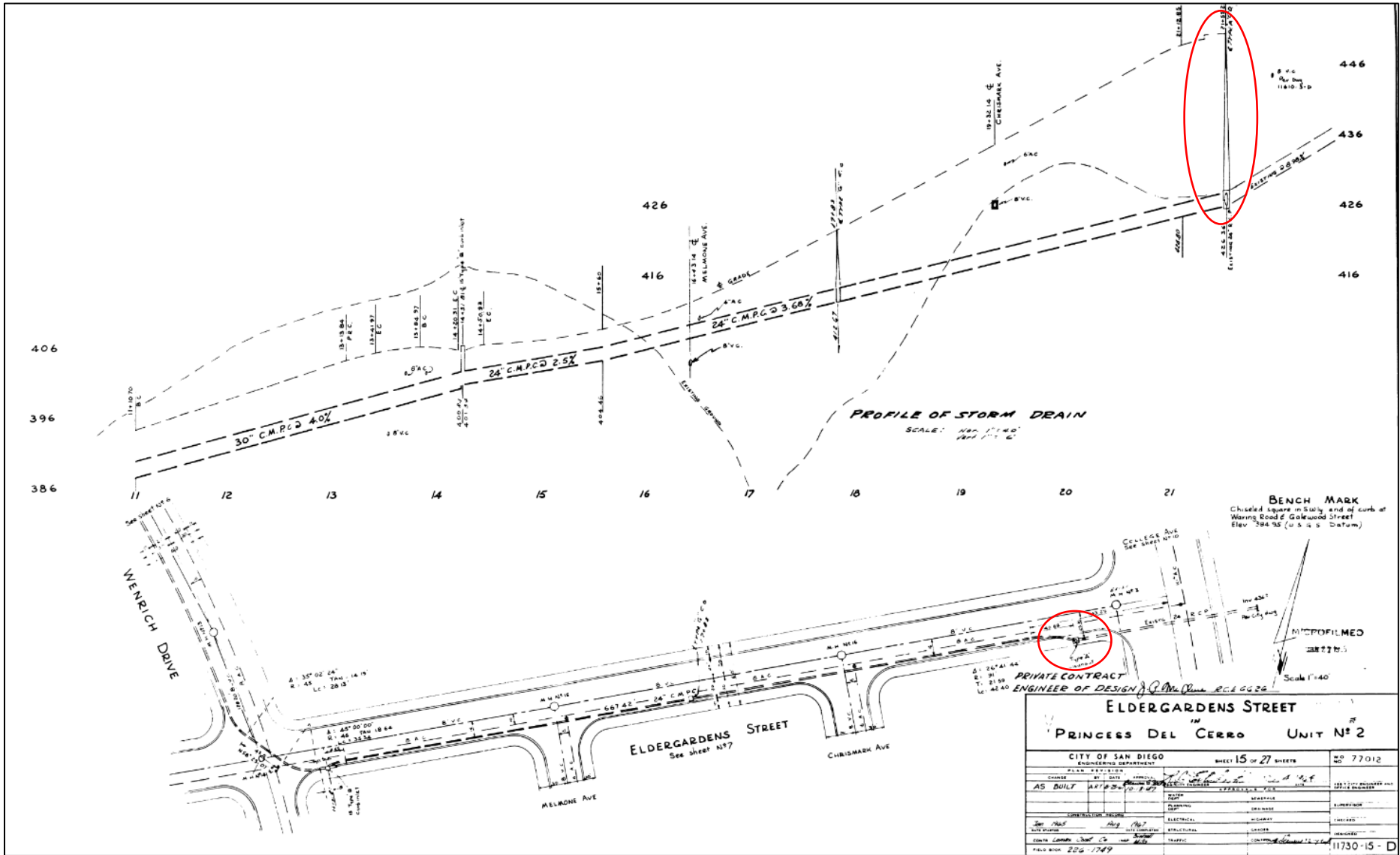
Figure 8 - As-Built, Area of Concern circled in Red (11730-15-D)
