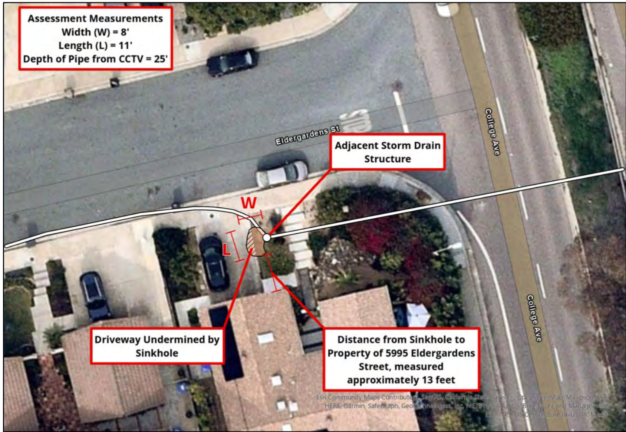
Figure 1 - Site Map Exhibit
