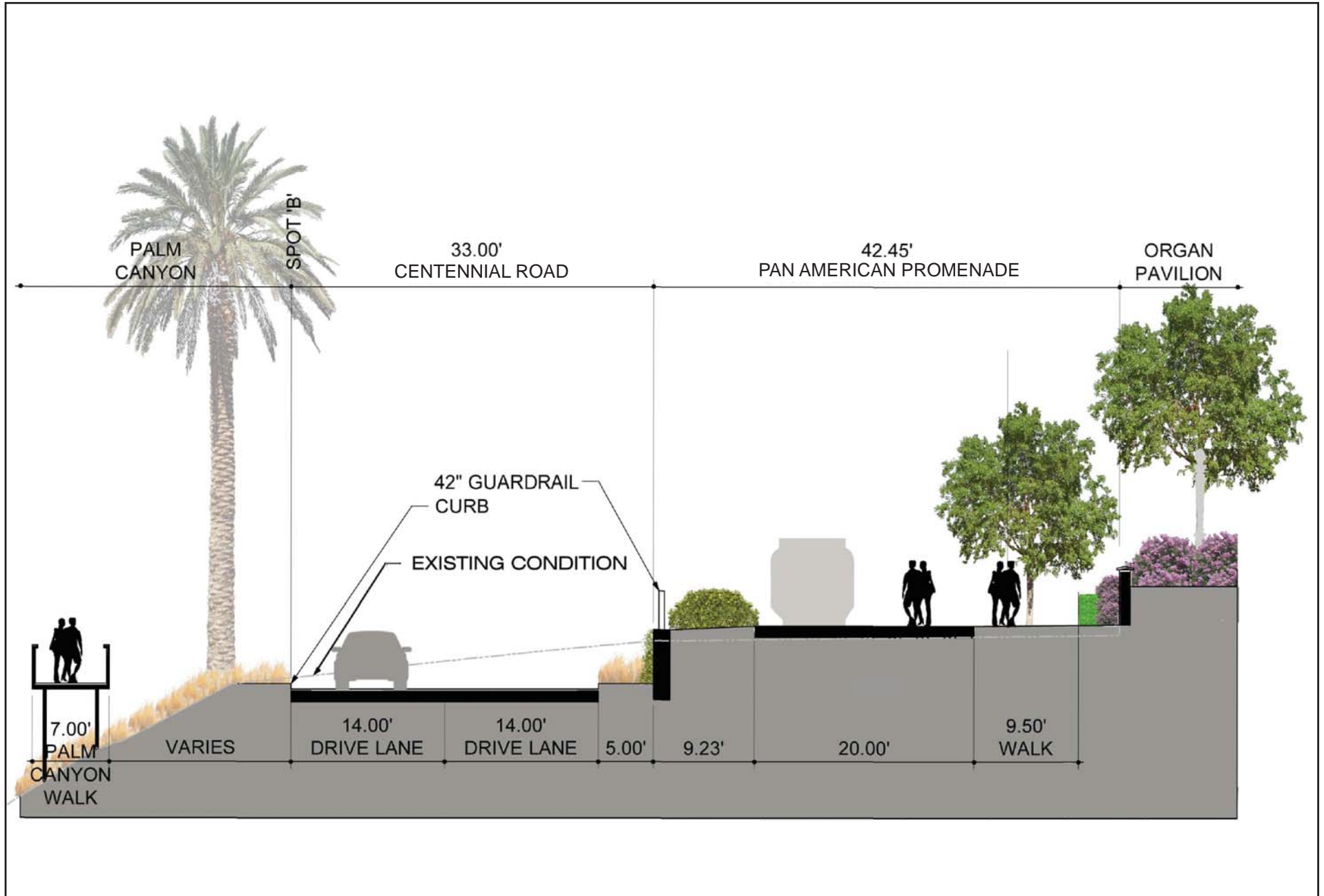
FIGURE 3-16 Conceptual Cross Section of Reconfigured Pan American Promenade and Palm Canyon Walkway (Revised)
