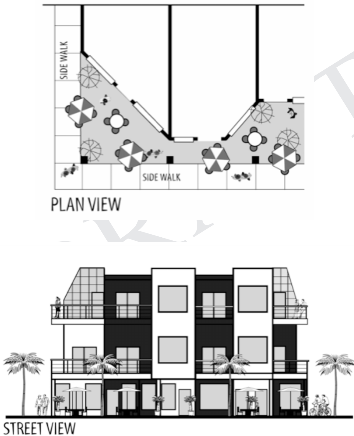
Figure 4-3 Chamfered Corners with outdoor seating
