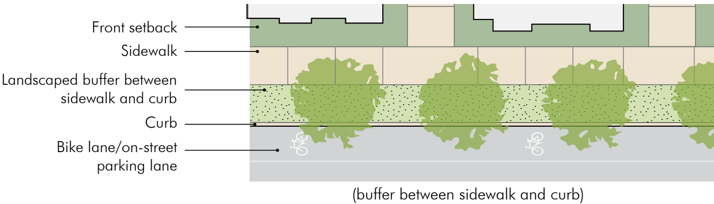
Figure 19: Noncontiguous Sidewalk
