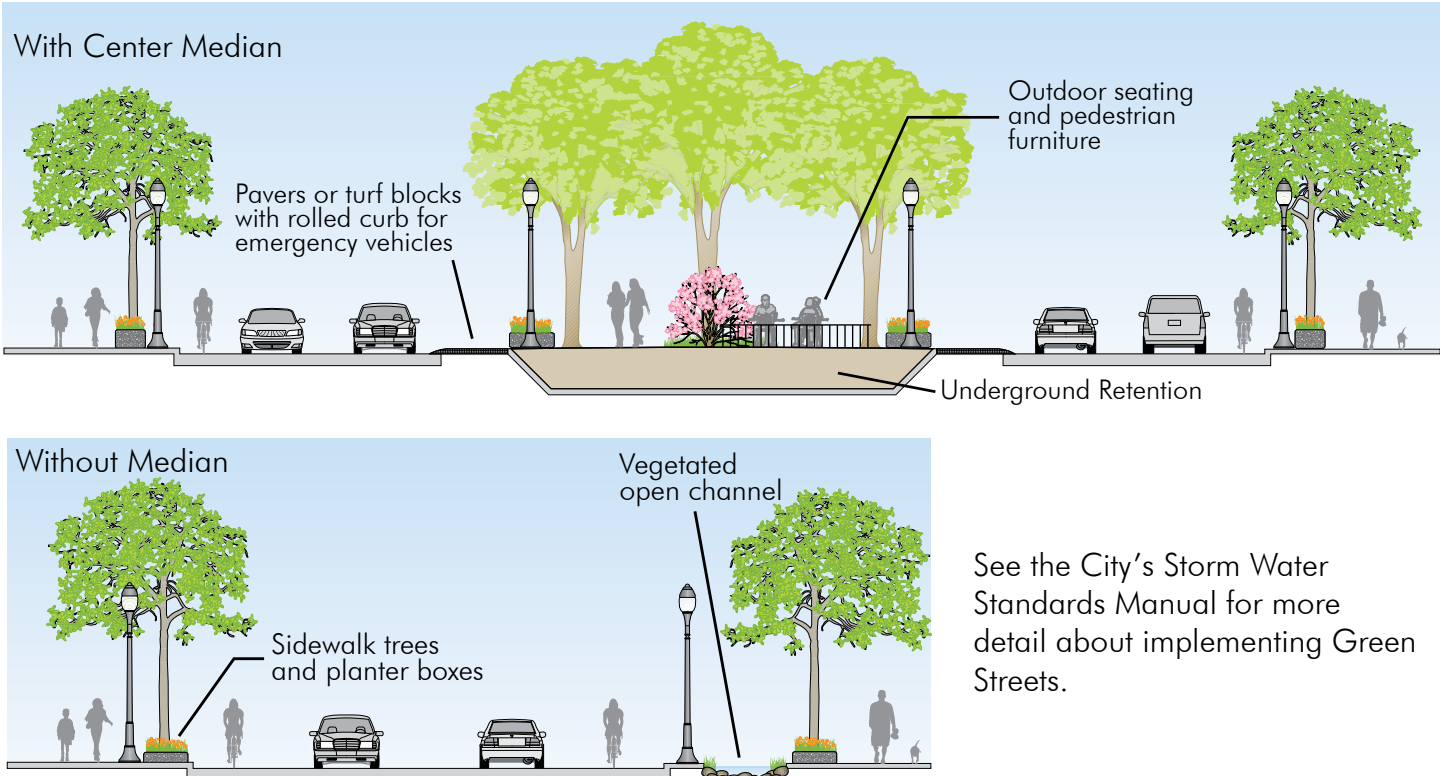
Figure 23: Green Streets
