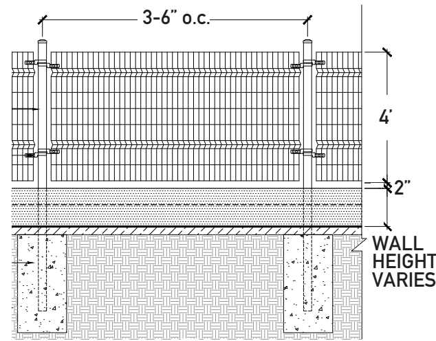
ELEVATION PLAY AREA ENCLOSURE Omega
