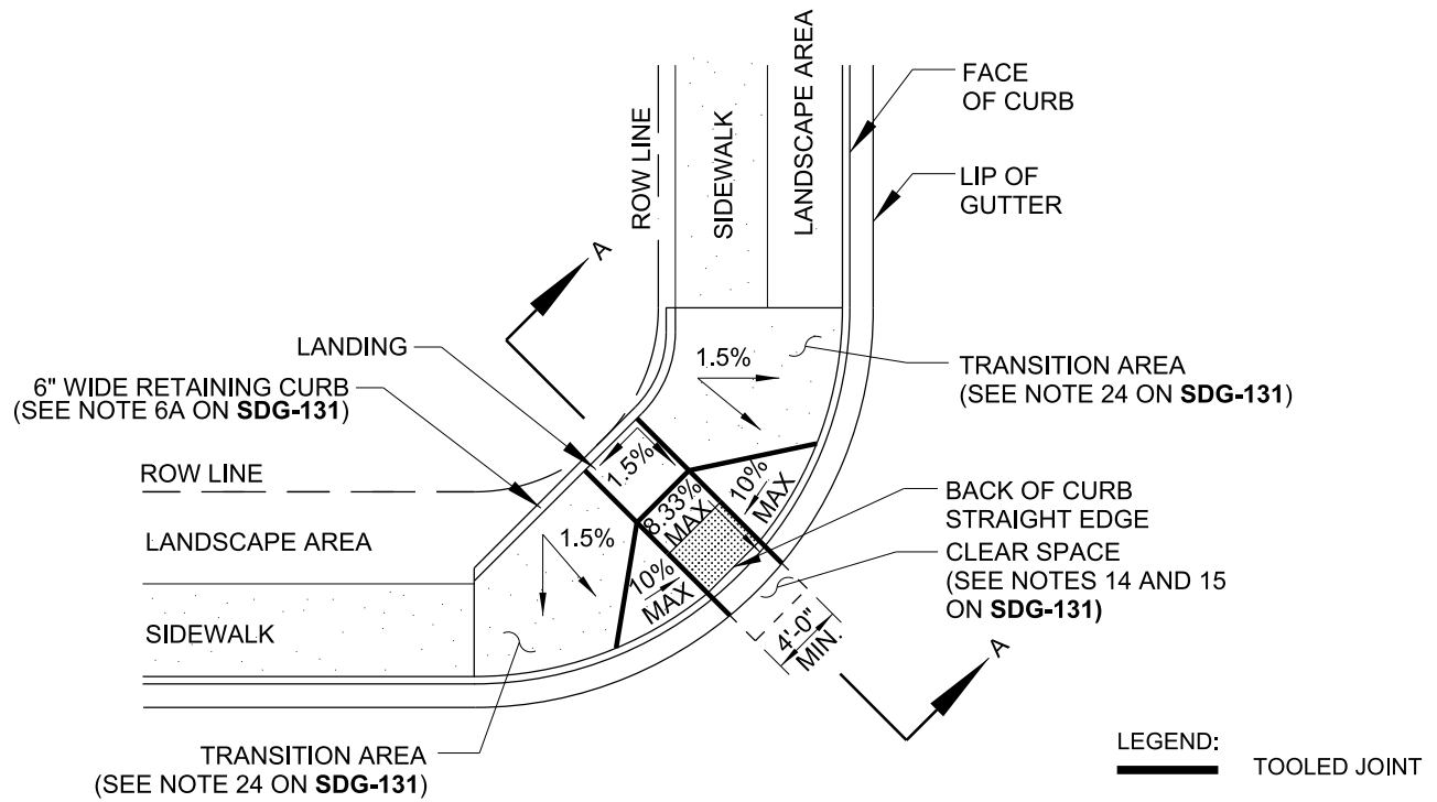
PLAN - TYPE A
