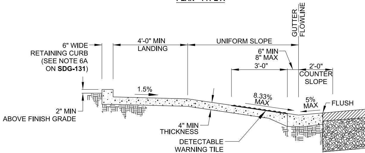
PLAN - TYPE A
