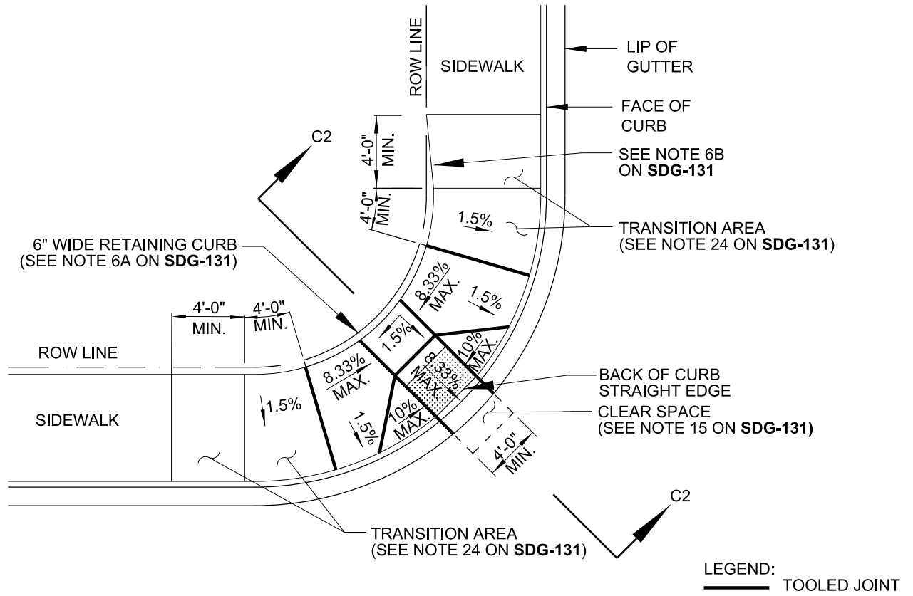
PLAN - TYPE C2
