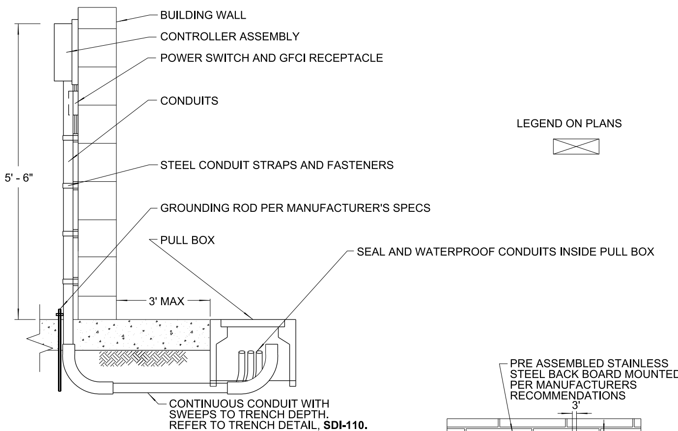
SIDE VIEW
