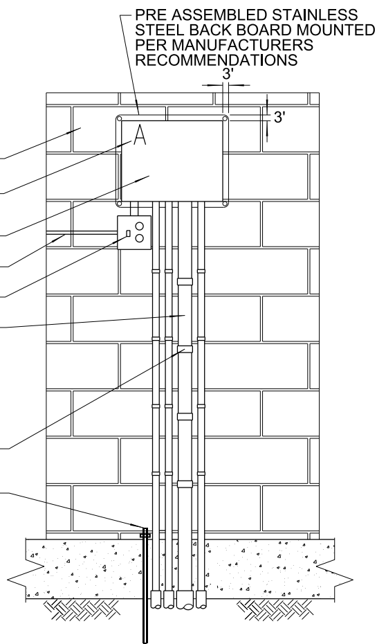
FRONT VIEW
