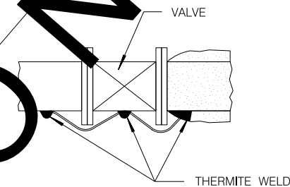
BONDING STRAP INSTALLED ON VALVE
