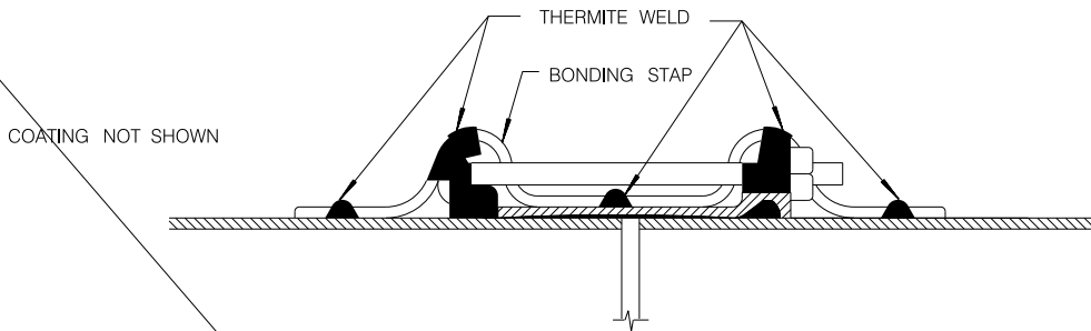
BONDING STRAP INSTALLED ON SLEEVE-TYPE COUPLING
