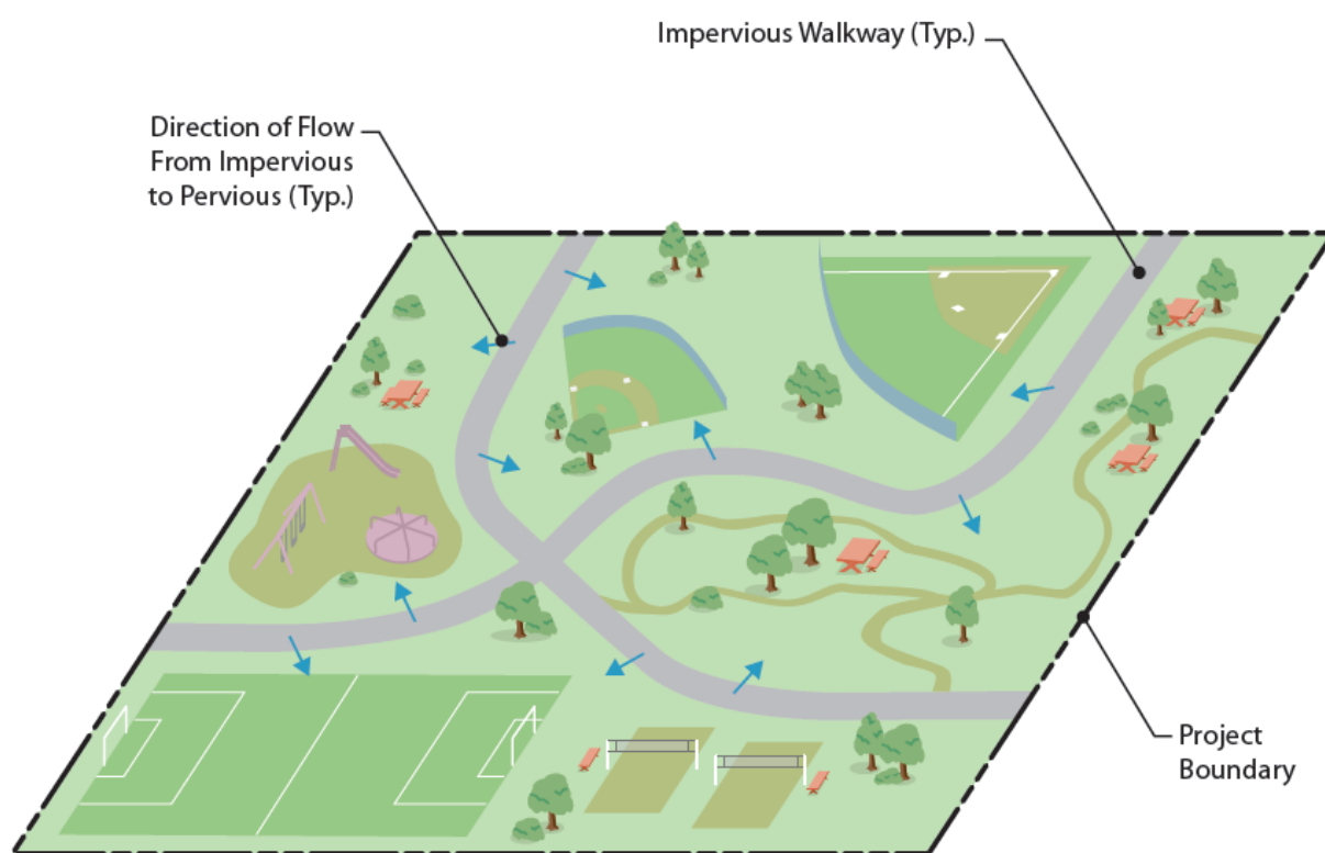
Figure 5-4. Self-retaining Site
