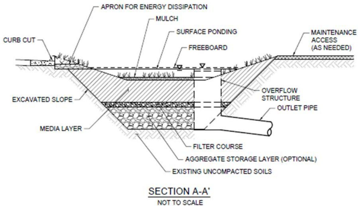
Figure E.14-1 : Typical Plan and Section View of a Bioretention BMP
